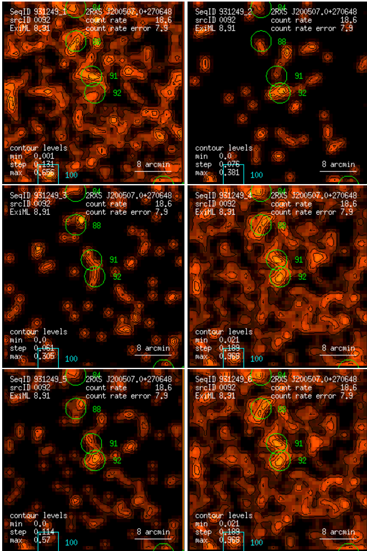
Figure 92: RASS 931249: detection 0092: band rate images, Gaussian filter: (1) PSPC channels 11 – 41, (2) 52 – 90, (3) 91 – 201, (4) 11 – 235, (5) 52 – 201, (6) 11 – 201. Broad band rates in counts/ks. Band rate contour levels in counts/ks/arcmin 2 .
