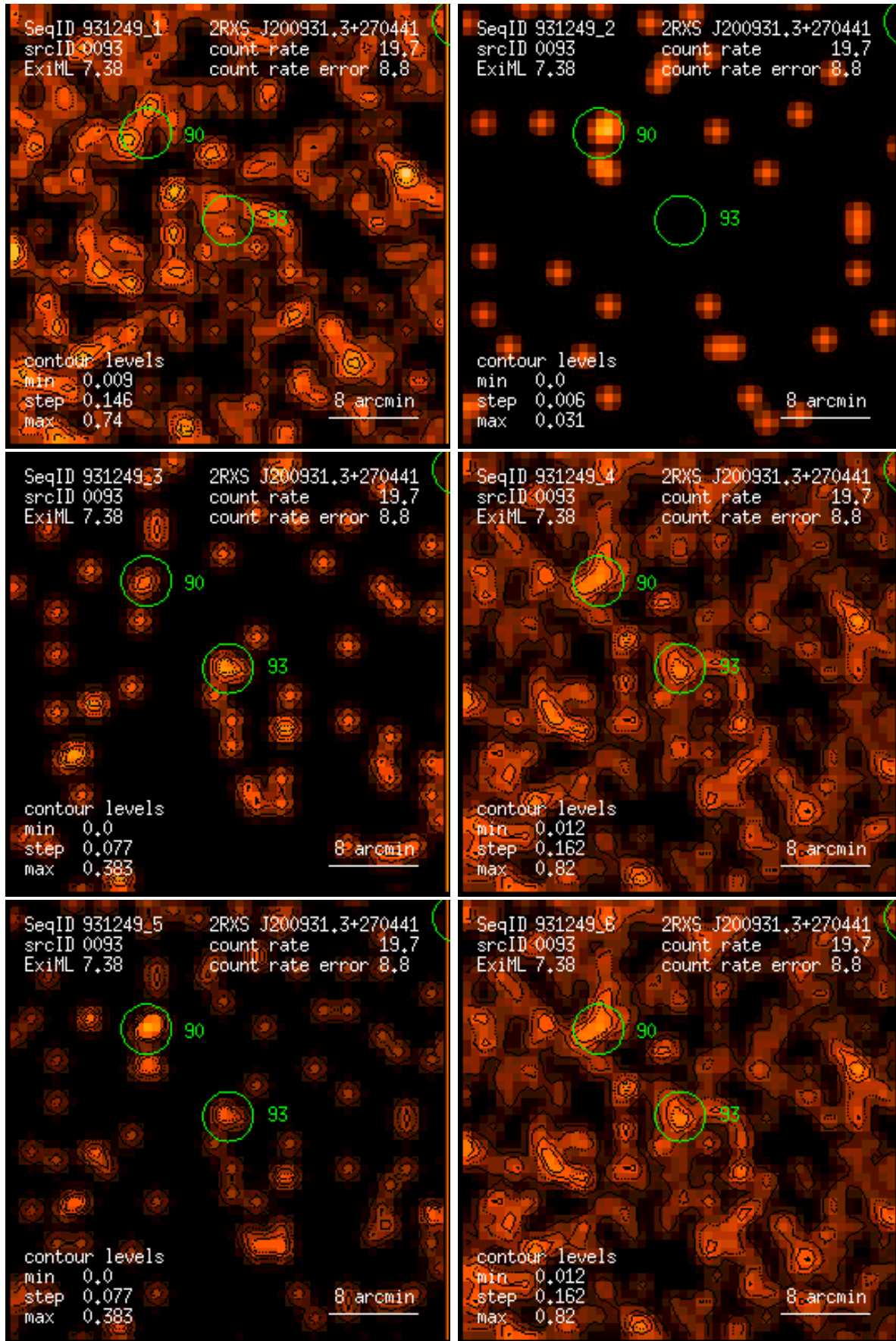
Figure 93: RASS 931249: detection 0093: band rate images, Gaussian filter: (1) PSPC channels 11 – 41, (2) 52 – 90, (3) 91 – 201, (4) 11 – 235, (5) 52 – 201, (6) 11 – 201. Broad band rates in counts/ks. Band rate contour levels in counts/ks/arcmin 2 .
