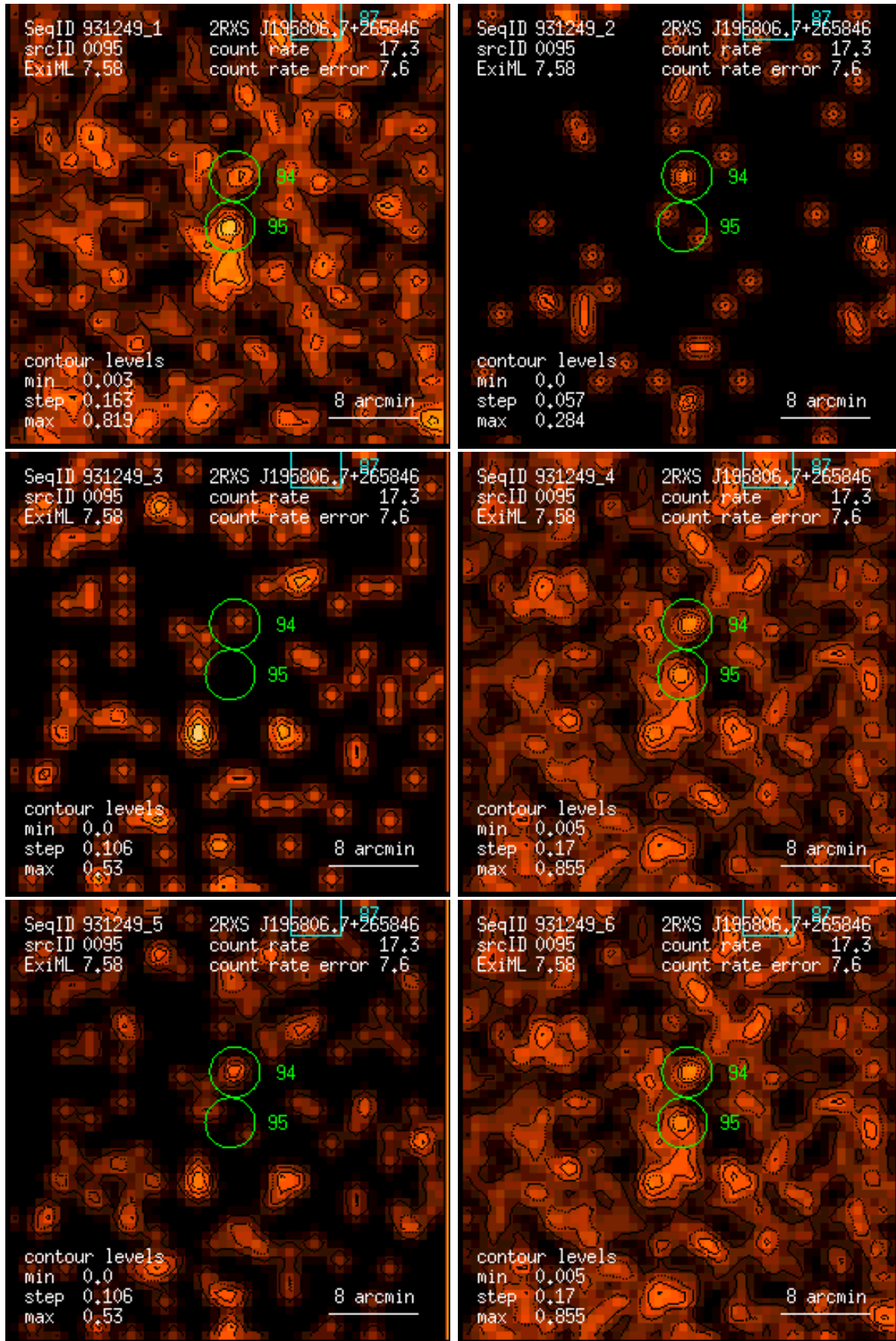
Figure 95: RASS 931249: detection 0095: band rate images, Gaussian filter: (1) PSPC channels 11 – 41, (2) 52 – 90, (3) 91 – 201, (4) 11 – 235, (5) 52 – 201, (6) 11 – 201. Broad band rates in counts/ks. Band rate contour levels in counts/ks/arcmin 2 .
