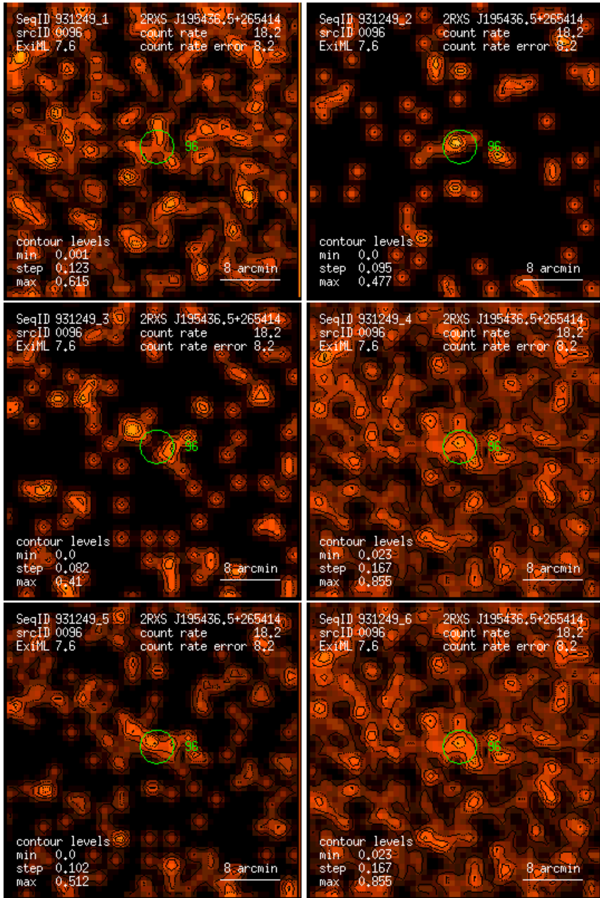
Figure 96: RASS 931249: detection 0096: band rate images, Gaussian filter: (1) PSPC channels 11 – 41, (2) 52 – 90, (3) 91 – 201, (4) 11 – 235, (5) 52 – 201, (6) 11 – 201. Broad band rates in counts/ks. Band rate contour levels in counts/ks/arcmin 2 .
