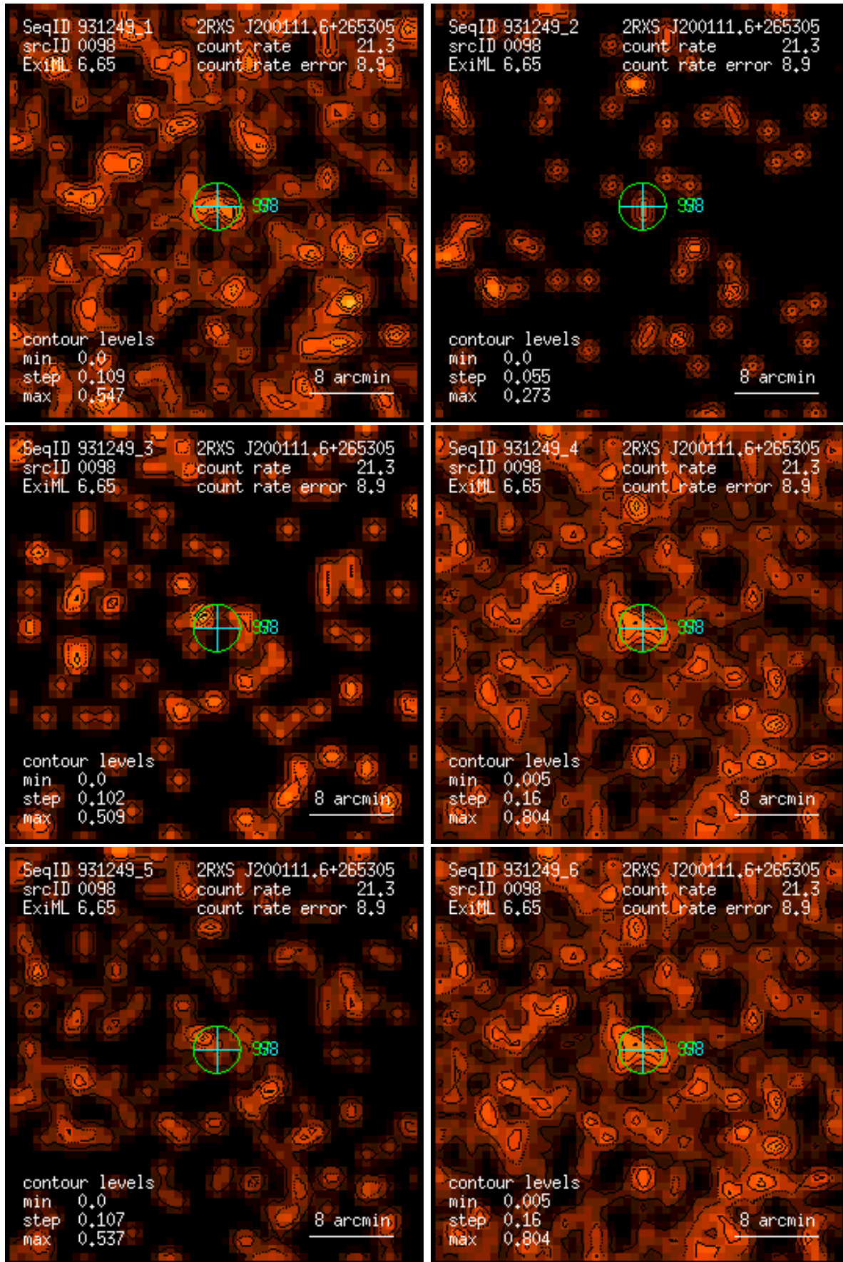
Figure 98: RASS 931249: detection 0098: band rate images, Gaussian filter: (1) PSPC channels 11 – 41, (2) 52 – 90, (3) 91 – 201, (4) 11 – 235, (5) 52 – 201, (6) 11 – 201. Broad band rates in counts/ks. Band rate contour levels in counts/ks/arcmin 2 .
