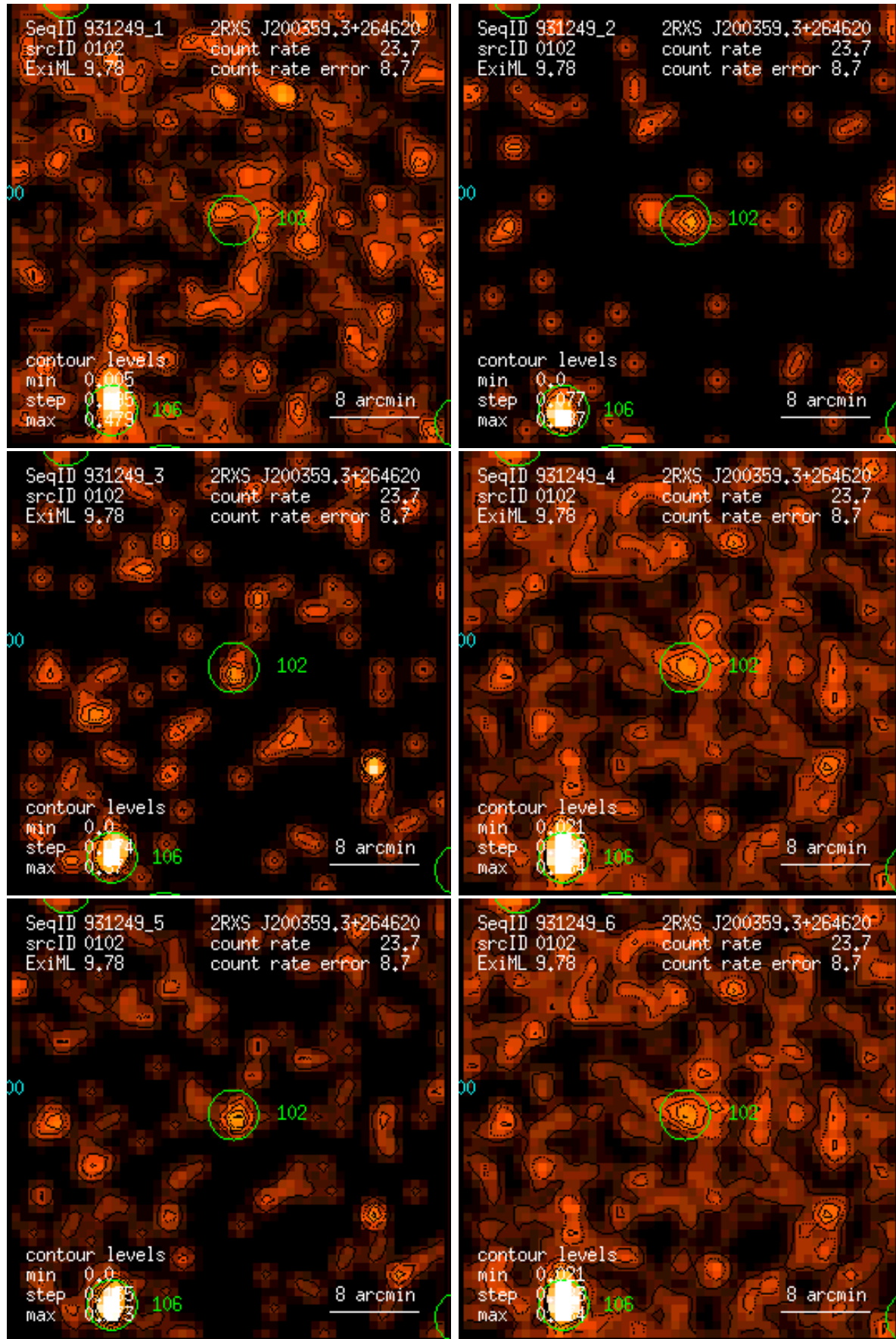
Figure 102: RASS 931249: detection 0102: band rate images, Gaussian filter: (1) PSPC channels 11 – 41, (2) 52 – 90, (3) 91 – 201, (4) 11 – 235, (5) 52 – 201, (6) 11 – 201. Broad band rates in counts/ks. Band rate contour levels in counts/ks/arcmin 2 .
