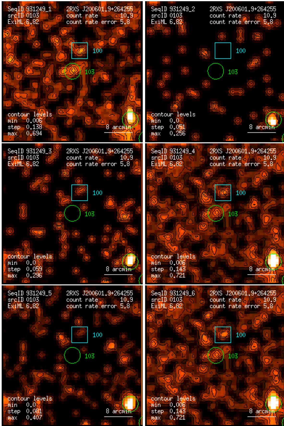
Figure 103: RASS 931249: detection 0103: band rate images, Gaussian filter: (1) PSPC channels 11 – 41, (2) 52 – 90, (3) 91 – 201, (4) 11 – 235, (5) 52 – 201, (6) 11 – 201. Broad band rates in counts/ks. Band rate contour levels in counts/ks/arcmin 2 .
