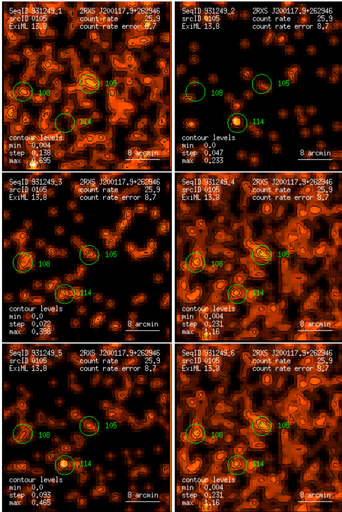
Figure 105: RASS 931249: detection 0105: band rate images, Gaussian filter: (1) PSPC channels 11 – 41, (2) 52 – 90, (3) 91 – 201, (4) 11 – 235, (5) 52 – 201, (6) 11 – 201. Broad band rates in counts/ks. Band rate contour levels in counts/ks/arcmin 2 .
