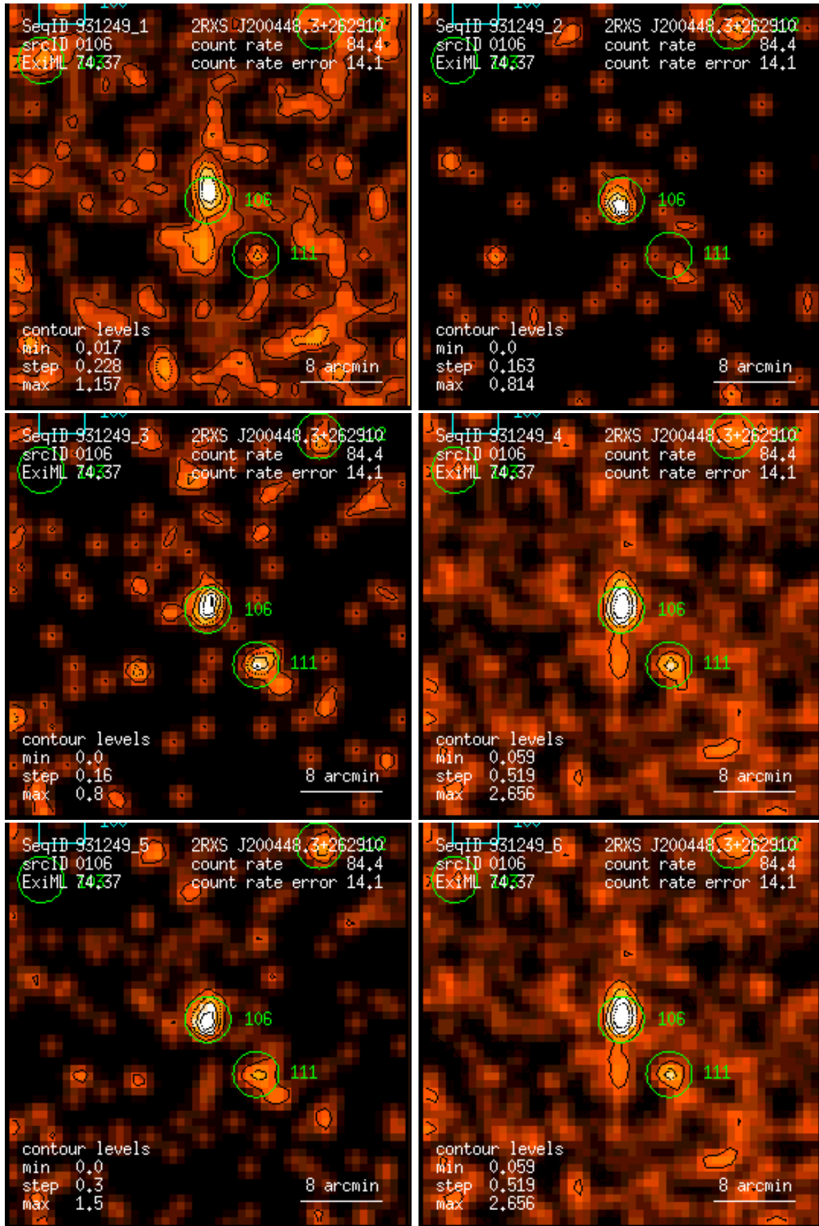
Figure 106: RASS 931249: detection 0106: band rate images, Gaussian filter: (1) PSPC channels 11 – 41, (2) 52 – 90, (3) 91 – 201, (4) 11 – 235, (5) 52 – 201, (6) 11 – 201. Broad band rates in counts/ks. Band rate contour levels in counts/ks/arcmin 2 .
