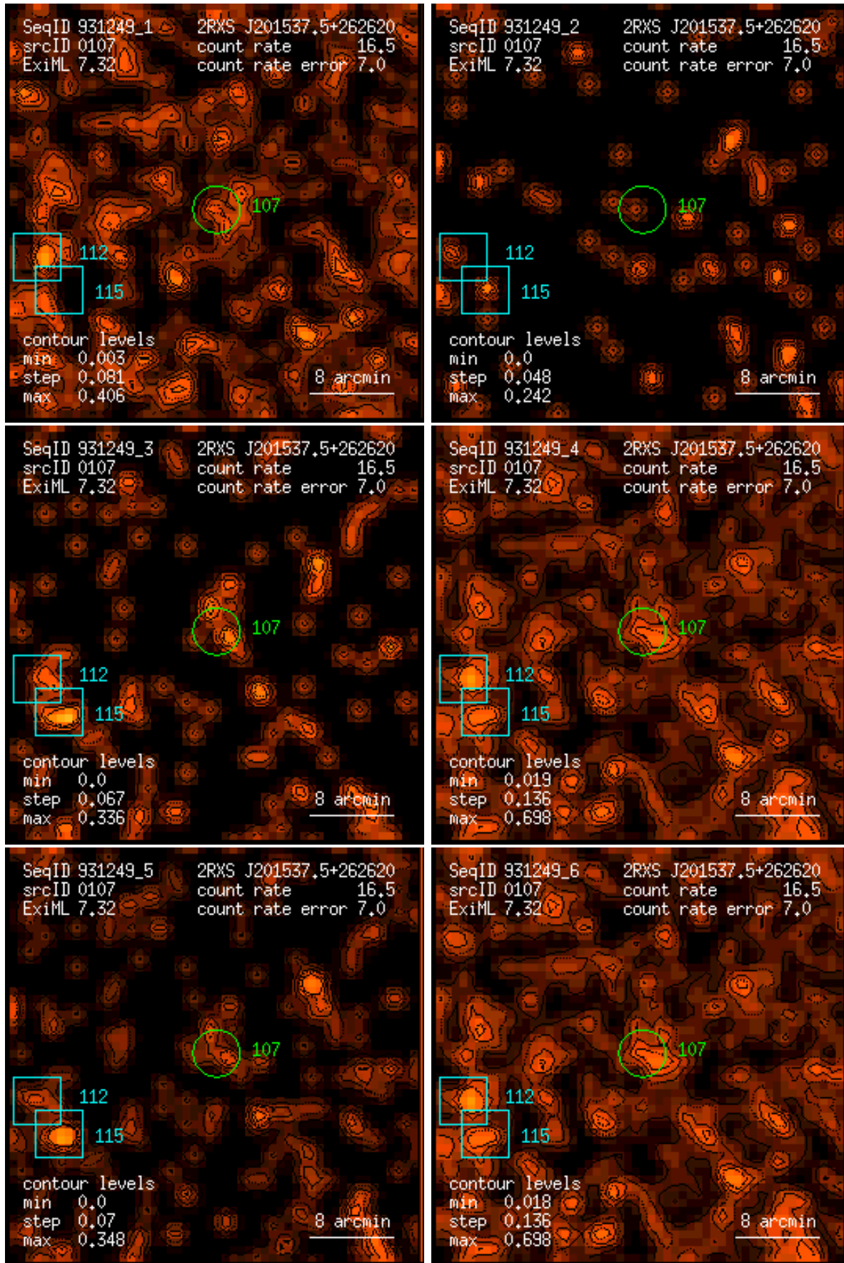
Figure 107: RASS 931249: detection 0107: band rate images, Gaussian filter: (1) PSPC channels 11 – 41, (2) 52 – 90, (3) 91 – 201, (4) 11 – 235, (5) 52 – 201, (6) 11 – 201. Broad band rates in counts/ks. Band rate contour levels in counts/ks/arcmin 2 .
