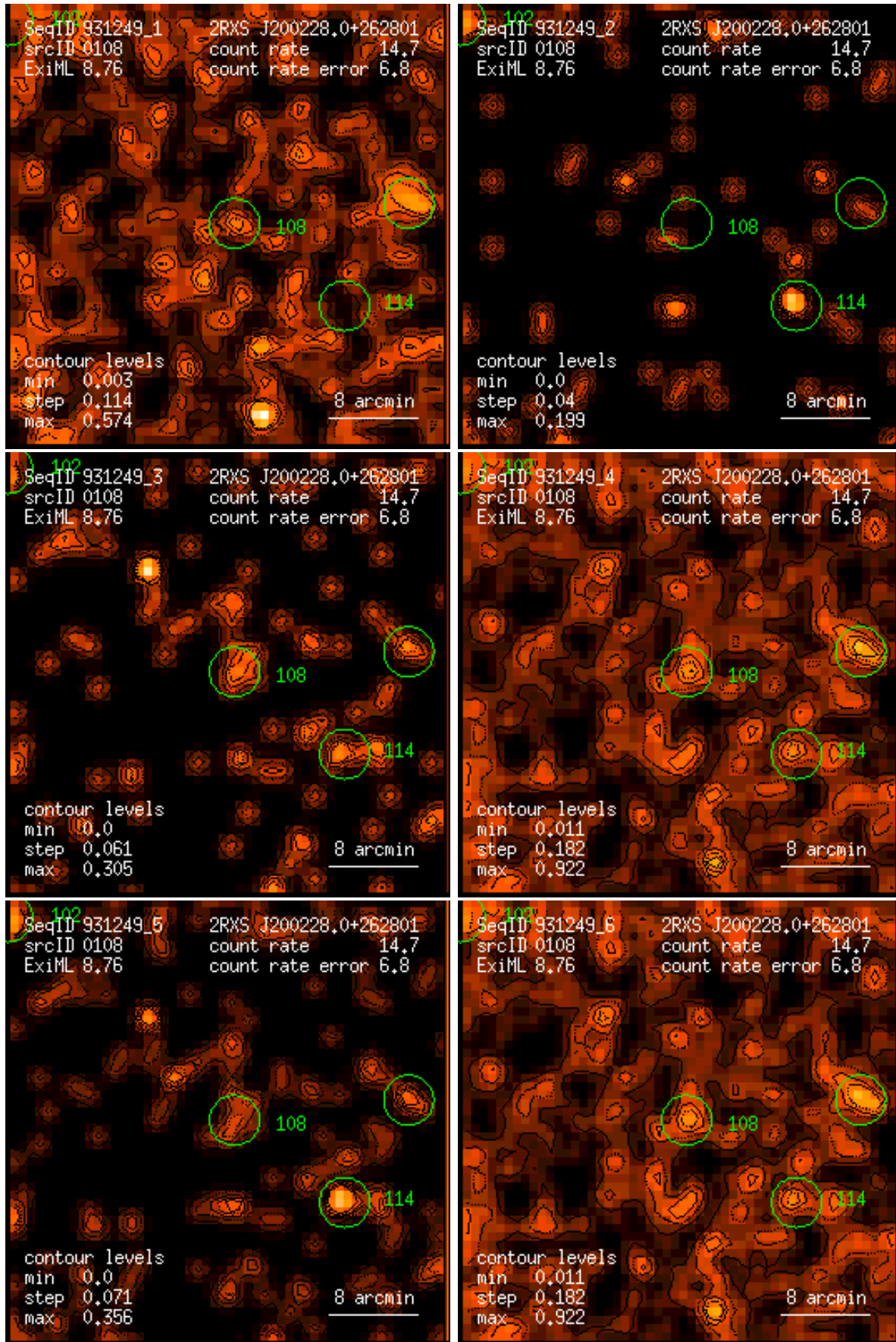
Figure 108: RASS 931249: detection 0108: band rate images, Gaussian filter: (1) PSPC channels 11 – 41, (2) 52 – 90, (3) 91 – 201, (4) 11 – 235, (5) 52 – 201, (6) 11 – 201. Broad band rates in counts/ks. Band rate contour levels in counts/ks/arcmin 2 .
