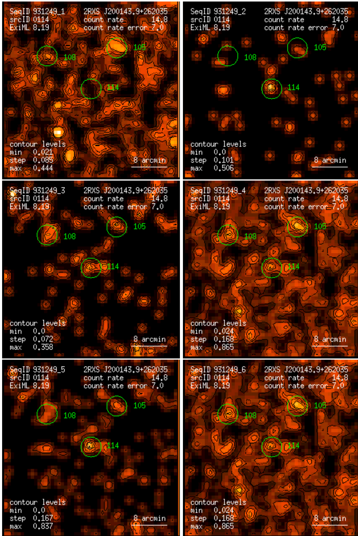
Figure 114: RASS 931249: detection 0114: band rate images, Gaussian filter: (1) PSPC channels 11 – 41, (2) 52 – 90, (3) 91 – 201, (4) 11 – 235, (5) 52 – 201, (6) 11 – 201. Broad band rates in counts/ks. Band rate contour levels in counts/ks/arcmin 2 .
