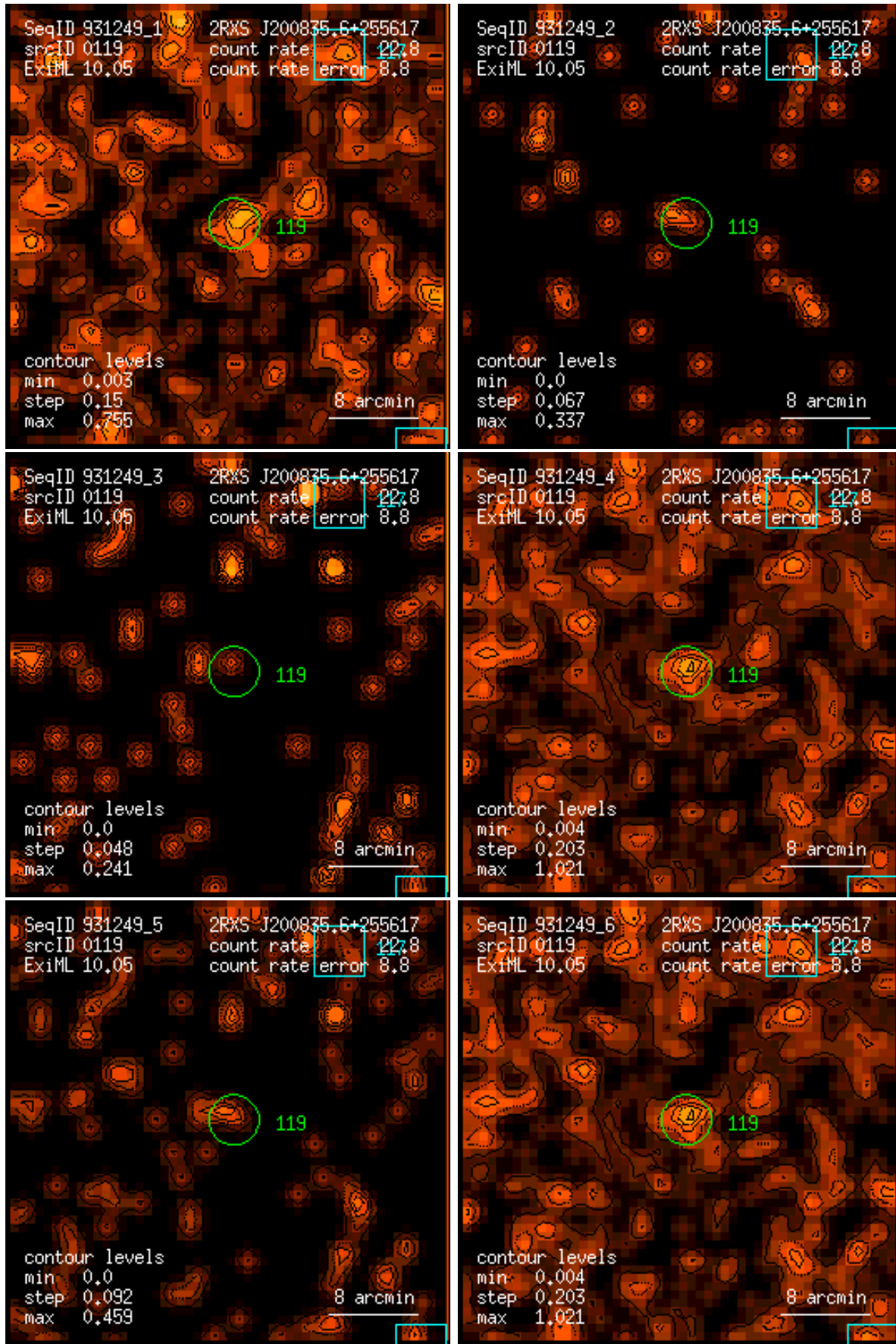
Figure 119: RASS 931249: detection 0119: band rate images, Gaussian filter: (1) PSPC channels 11 – 41, (2) 52 – 90, (3) 91 – 201, (4) 11 – 235, (5) 52 – 201, (6) 11 – 201. Broad band rates in counts/ks. Band rate contour levels in counts/ks/arcmin 2 .
