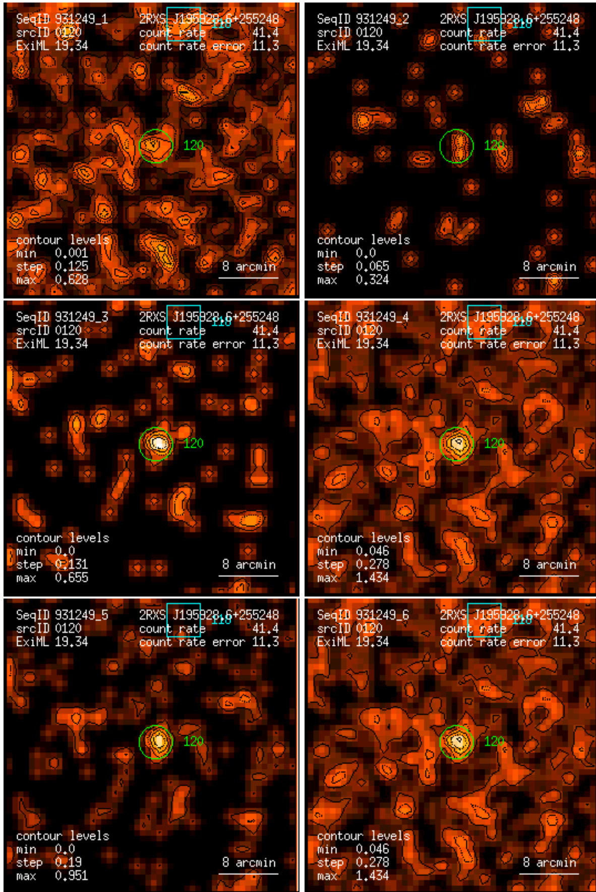
Figure 120: RASS 931249: detection 0120: band rate images, Gaussian filter: (1) PSPC channels 11 – 41, (2) 52 – 90, (3) 91 – 201, (4) 11 – 235, (5) 52 – 201, (6) 11 – 201. Broad band rates in counts/ks. Band rate contour levels in counts/ks/arcmin 2 .
