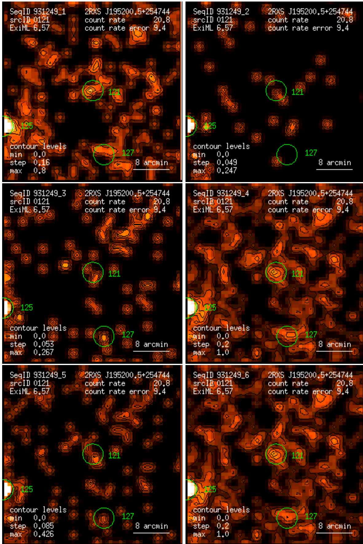
Figure 121: RASS 931249: detection 0121: band rate images, Gaussian filter: (1) PSPC channels 11 – 41, (2) 52 – 90, (3) 91 – 201, (4) 11 – 235, (5) 52 – 201, (6) 11 – 201. Broad band rates in counts/ks. Band rate contour levels in counts/ks/arcmin 2 .
