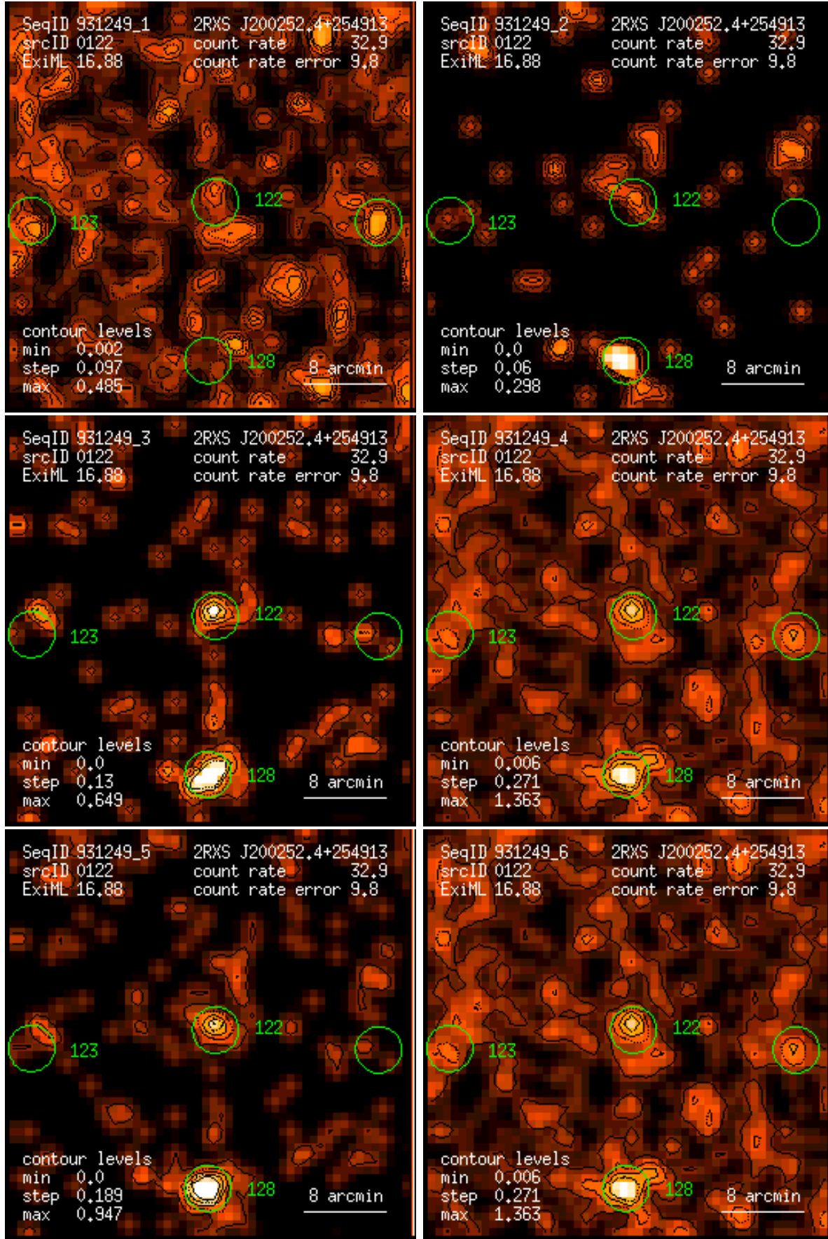
Figure 122: RASS 931249: detection 0122: band rate images, Gaussian filter: (1) PSPC channels 11 – 41, (2) 52 – 90, (3) 91 – 201, (4) 11 – 235, (5) 52 – 201, (6) 11 – 201. Broad band rates in counts/ks. Band rate contour levels in counts/ks/arcmin 2 .
