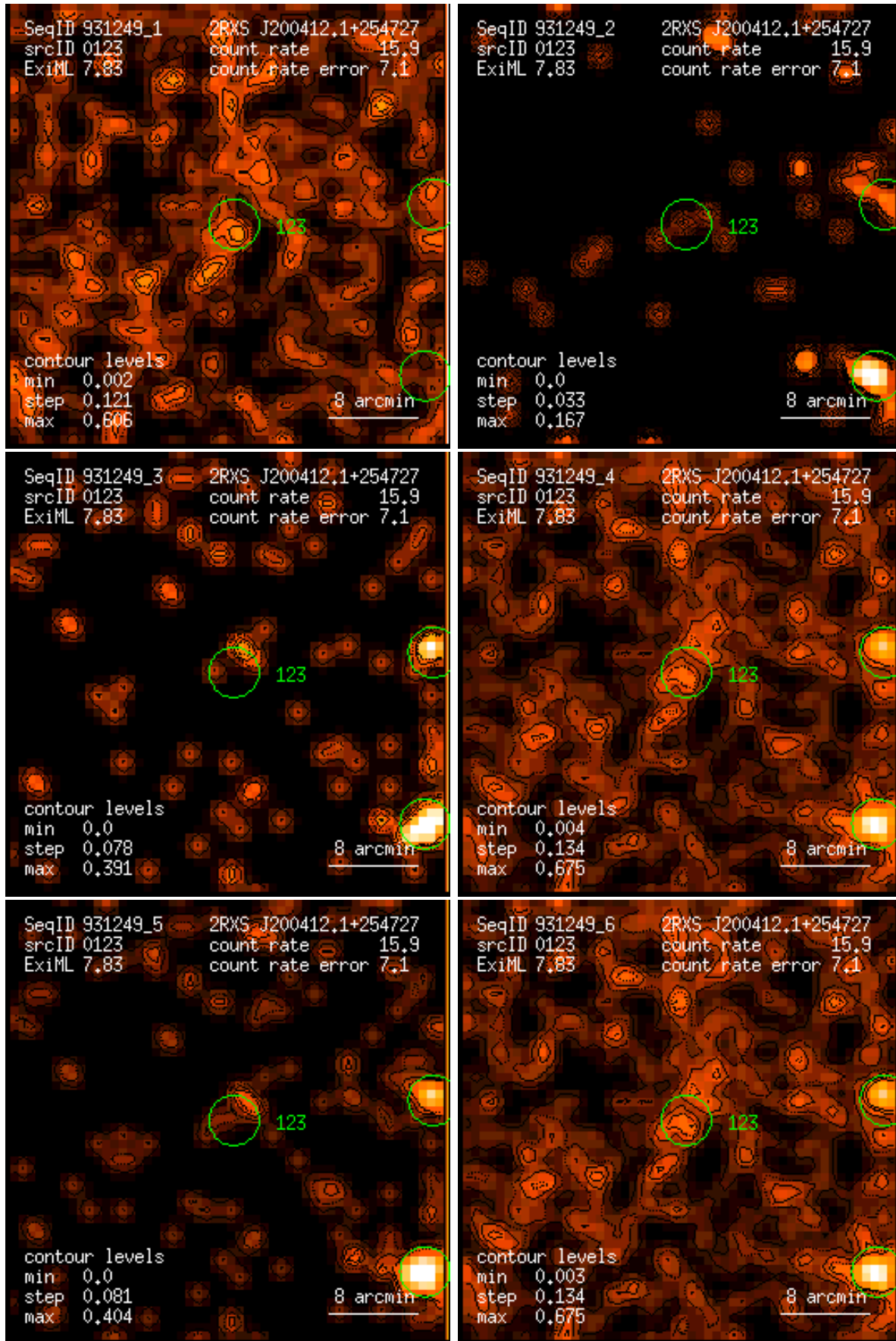
Figure 123: RASS 931249: detection 0123: band rate images, Gaussian filter: (1) PSPC channels 11 – 41, (2) 52 – 90, (3) 91 – 201, (4) 11 – 235, (5) 52 – 201, (6) 11 – 201. Broad band rates in counts/ks. Band rate contour levels in counts/ks/arcmin 2 .
