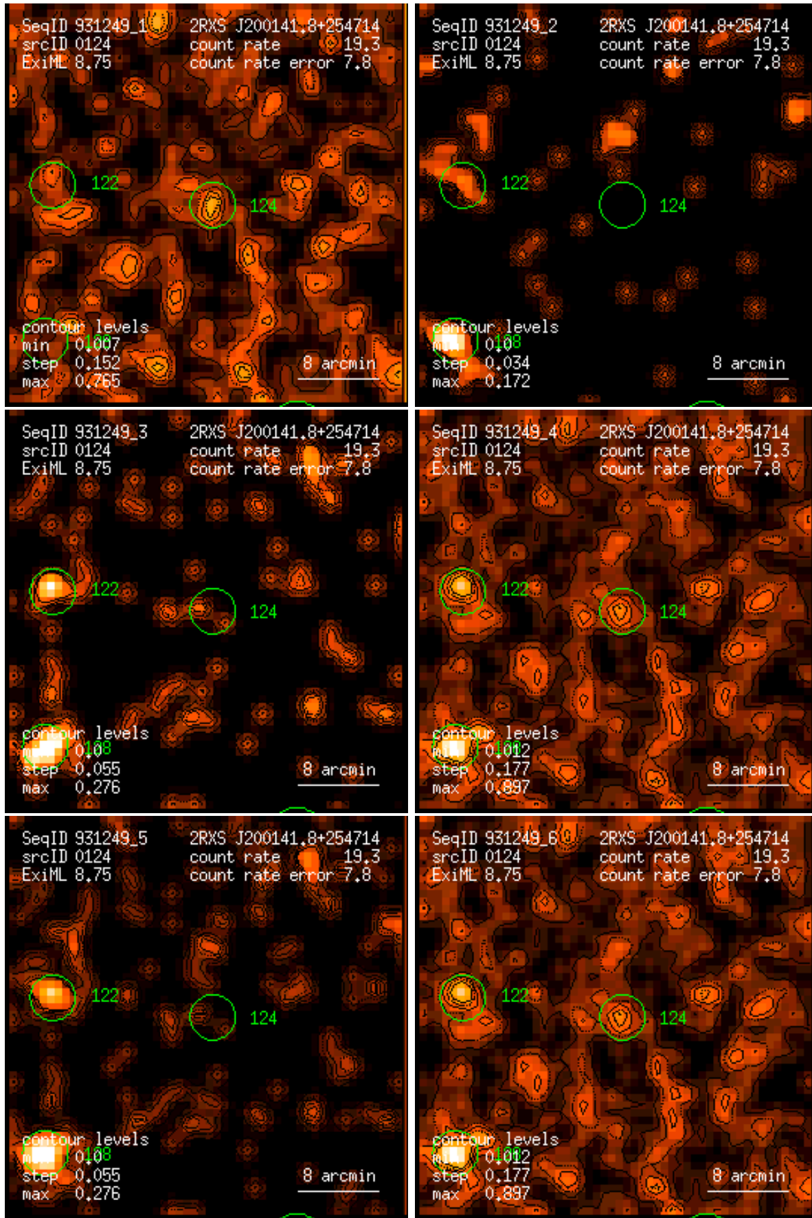
Figure 124: RASS 931249: detection 0124: band rate images, Gaussian filter: (1) PSPC channels 11 – 41, (2) 52 – 90, (3) 91 – 201, (4) 11 – 235, (5) 52 – 201, (6) 11 – 201. Broad band rates in counts/ks. Band rate contour levels in counts/ks/arcmin 2 .
