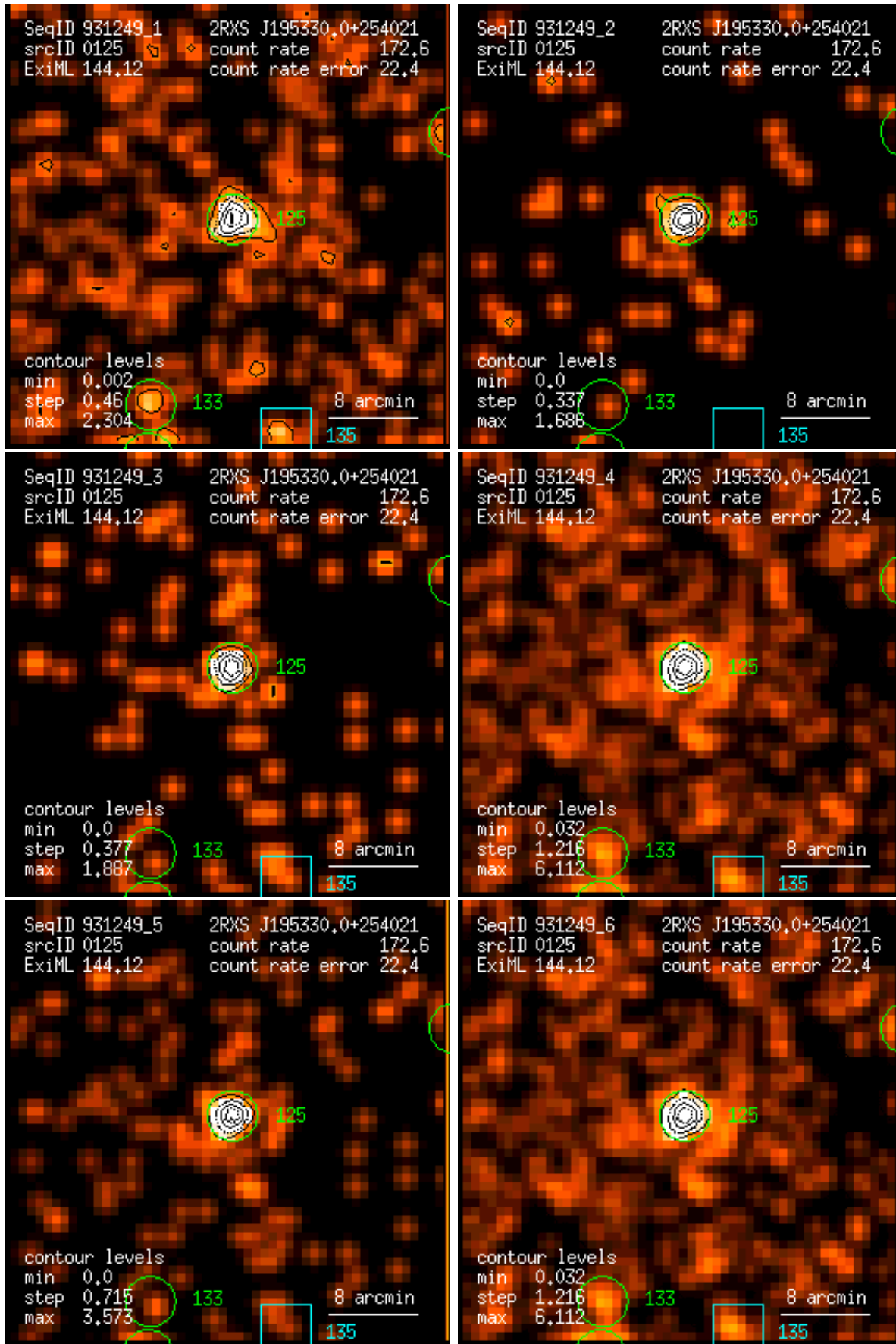
Figure 125: RASS 931249: detection 0125: band rate images, Gaussian filter: (1) PSPC channels 11 – 41, (2) 52 – 90, (3) 91 – 201, (4) 11 – 235, (5) 52 – 201, (6) 11 – 201. Broad band rates in counts/ks. Band rate contour levels in counts/ks/arcmin 2 .
