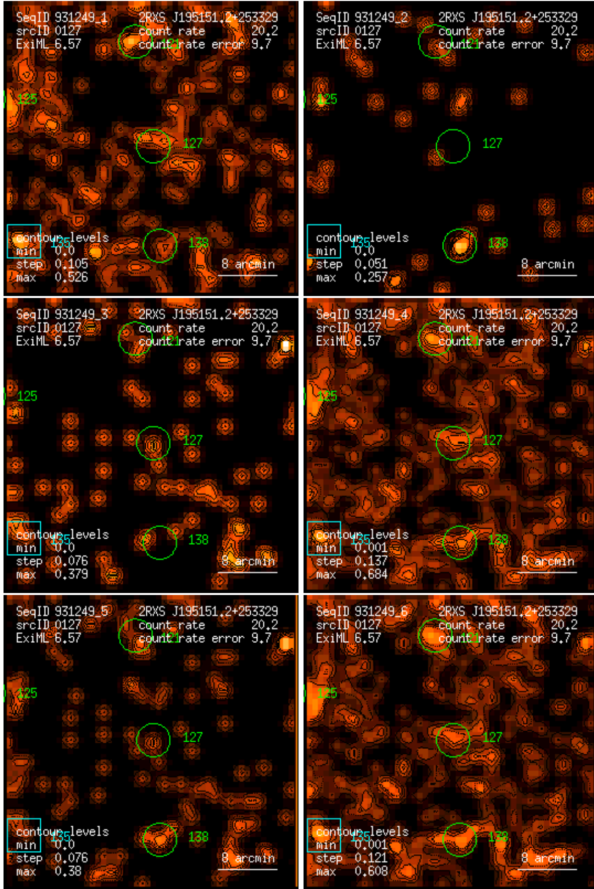
Figure 127: RASS 931249: detection 0127: band rate images, Gaussian filter: (1) PSPC channels 11 – 41, (2) 52 – 90, (3) 91 – 201, (4) 11 – 235, (5) 52 – 201, (6) 11 – 201. Broad band rates in counts/ks. Band rate contour levels in counts/ks/arcmin 2 .
