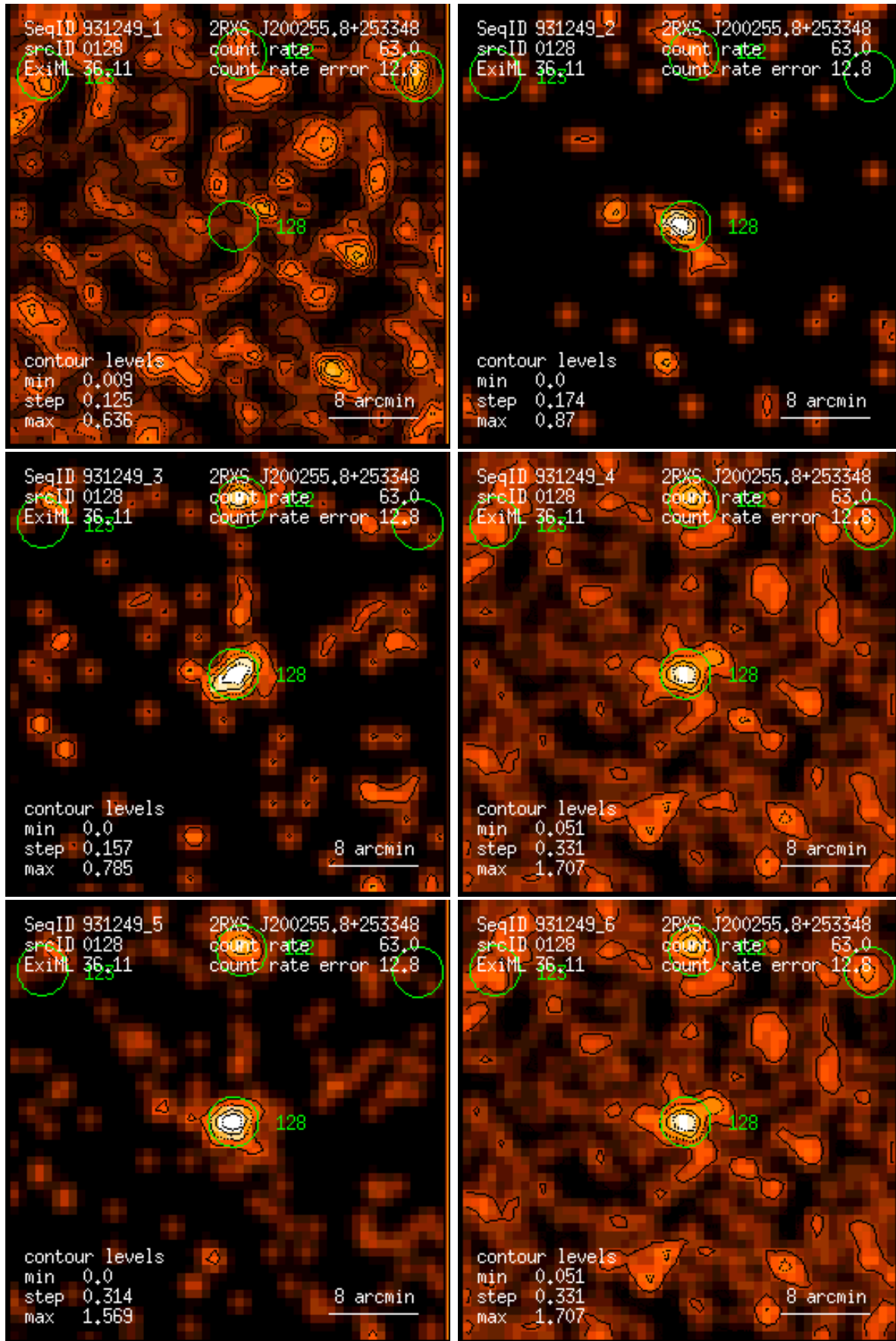
Figure 128: RASS 931249: detection 0128: band rate images, Gaussian filter: (1) PSPC channels 11 – 41, (2) 52 – 90, (3) 91 – 201, (4) 11 – 235, (5) 52 – 201, (6) 11 – 201. Broad band rates in counts/ks. Band rate contour levels in counts/ks/arcmin 2 .
