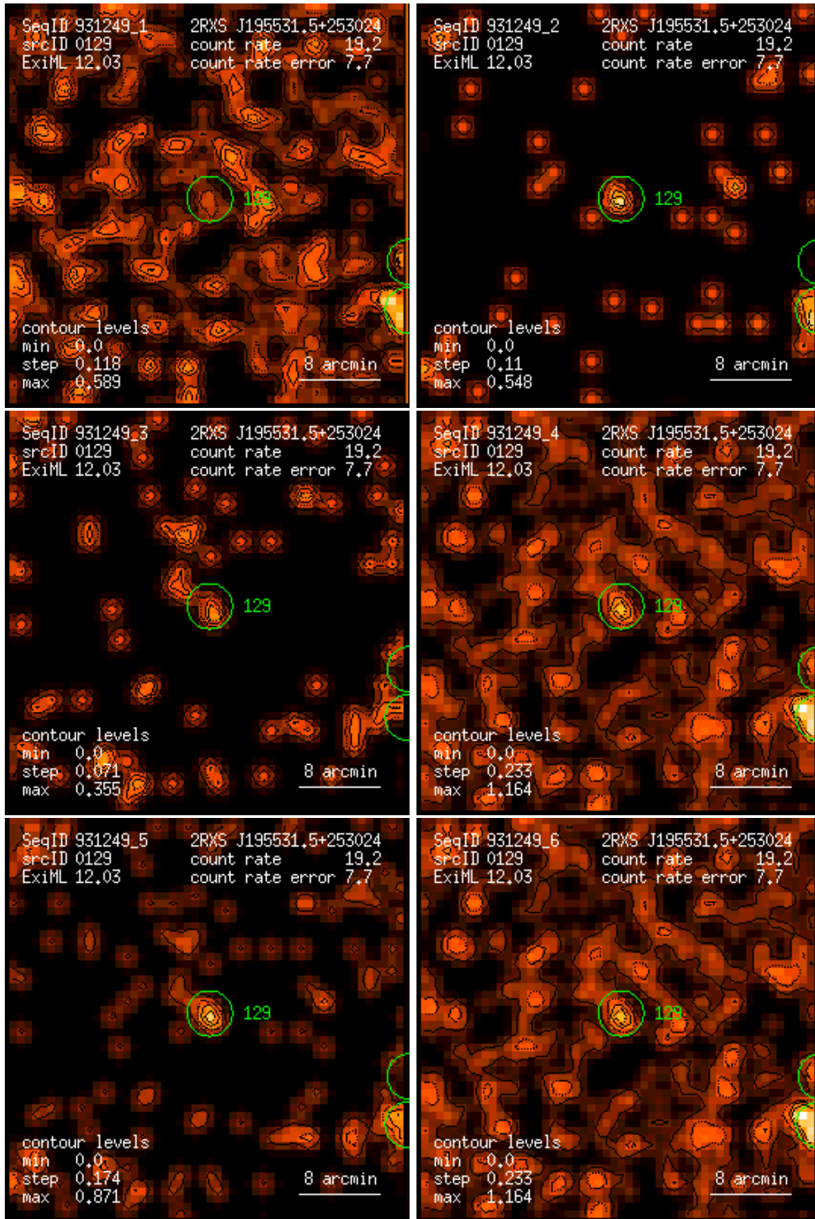
Figure 129: RASS 931249: detection 0129: band rate images, Gaussian filter: (1) PSPC channels 11 – 41, (2) 52 – 90, (3) 91 – 201, (4) 11 – 235, (5) 52 – 201, (6) 11 – 201. Broad band rates in counts/ks. Band rate contour levels in counts/ks/arcmin 2 .
