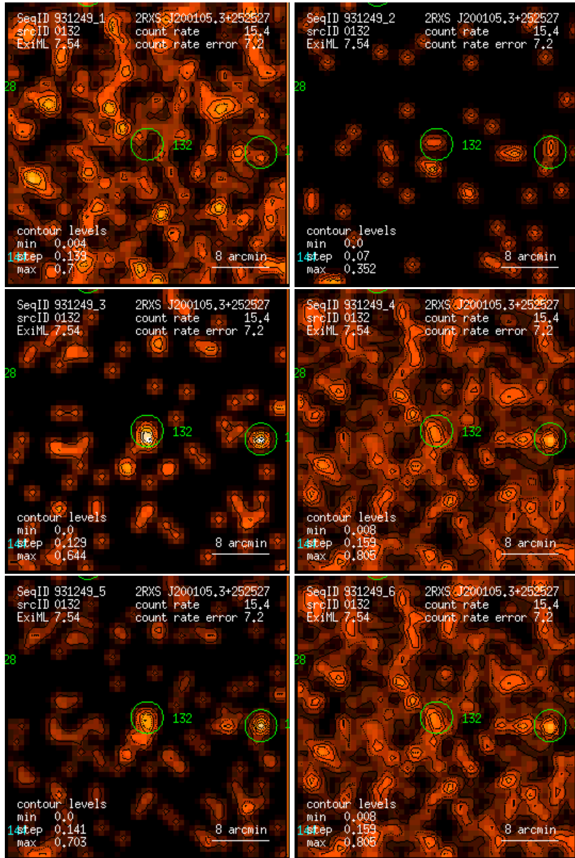
Figure 132: RASS 931249: detection 0132: band rate images, Gaussian filter: (1) PSPC channels 11 – 41, (2) 52 – 90, (3) 91 – 201, (4) 11 – 235, (5) 52 – 201, (6) 11 – 201. Broad band rates in counts/ks. Band rate contour levels in counts/ks/arcmin 2 .
