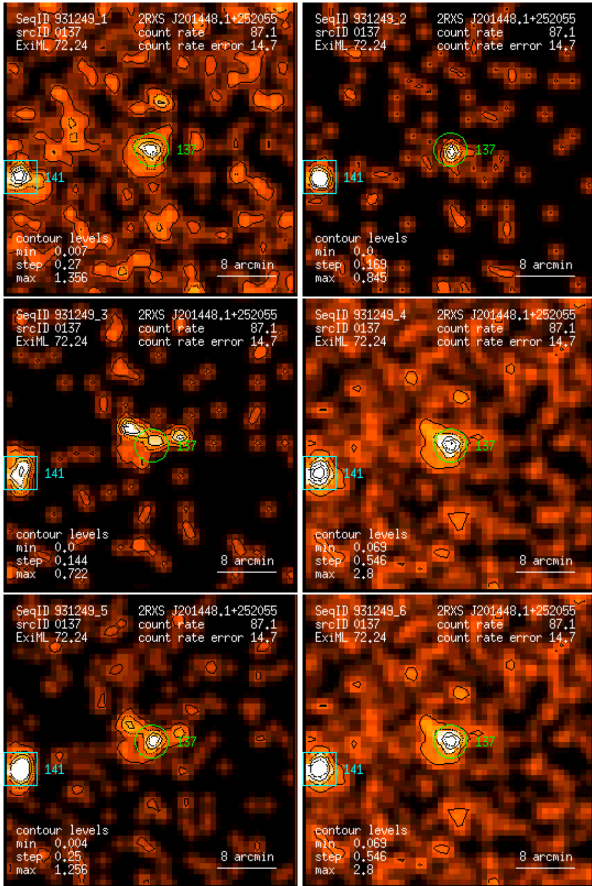
Figure 137: RASS 931249: detection 0137: band rate images, Gaussian filter: (1) PSPC channels 11 – 41, (2) 52 – 90, (3) 91 – 201, (4) 11 – 235, (5) 52 – 201, (6) 11 – 201. Broad band rates in counts/ks. Band rate contour levels in counts/ks/arcmin 2 .
