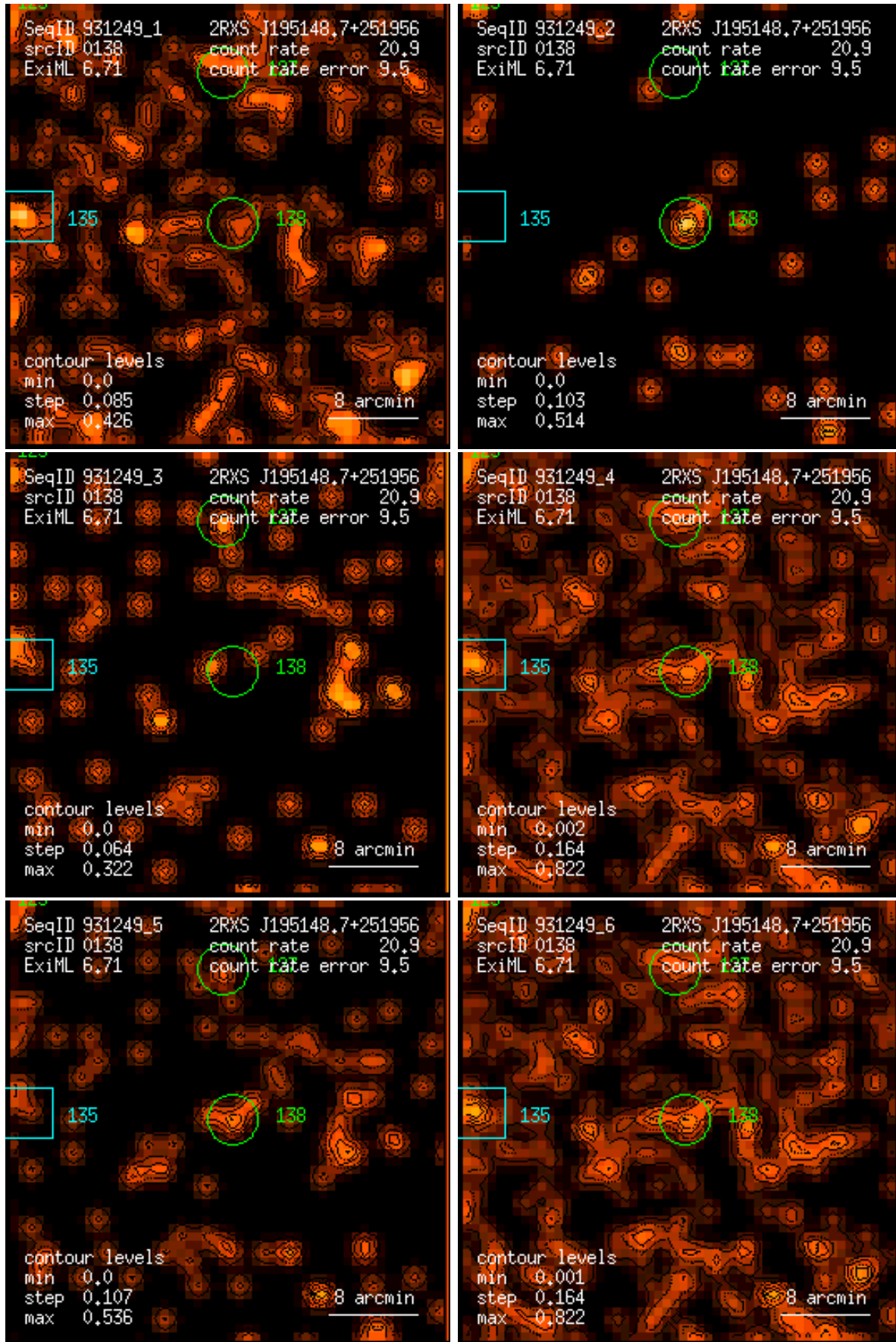
Figure 138: RASS 931249: detection 0138: band rate images, Gaussian filter: (1) PSPC channels 11 – 41, (2) 52 – 90, (3) 91 – 201, (4) 11 – 235, (5) 52 – 201, (6) 11 – 201. Broad band rates in counts/ks. Band rate contour levels in counts/ks/arcmin 2 .
