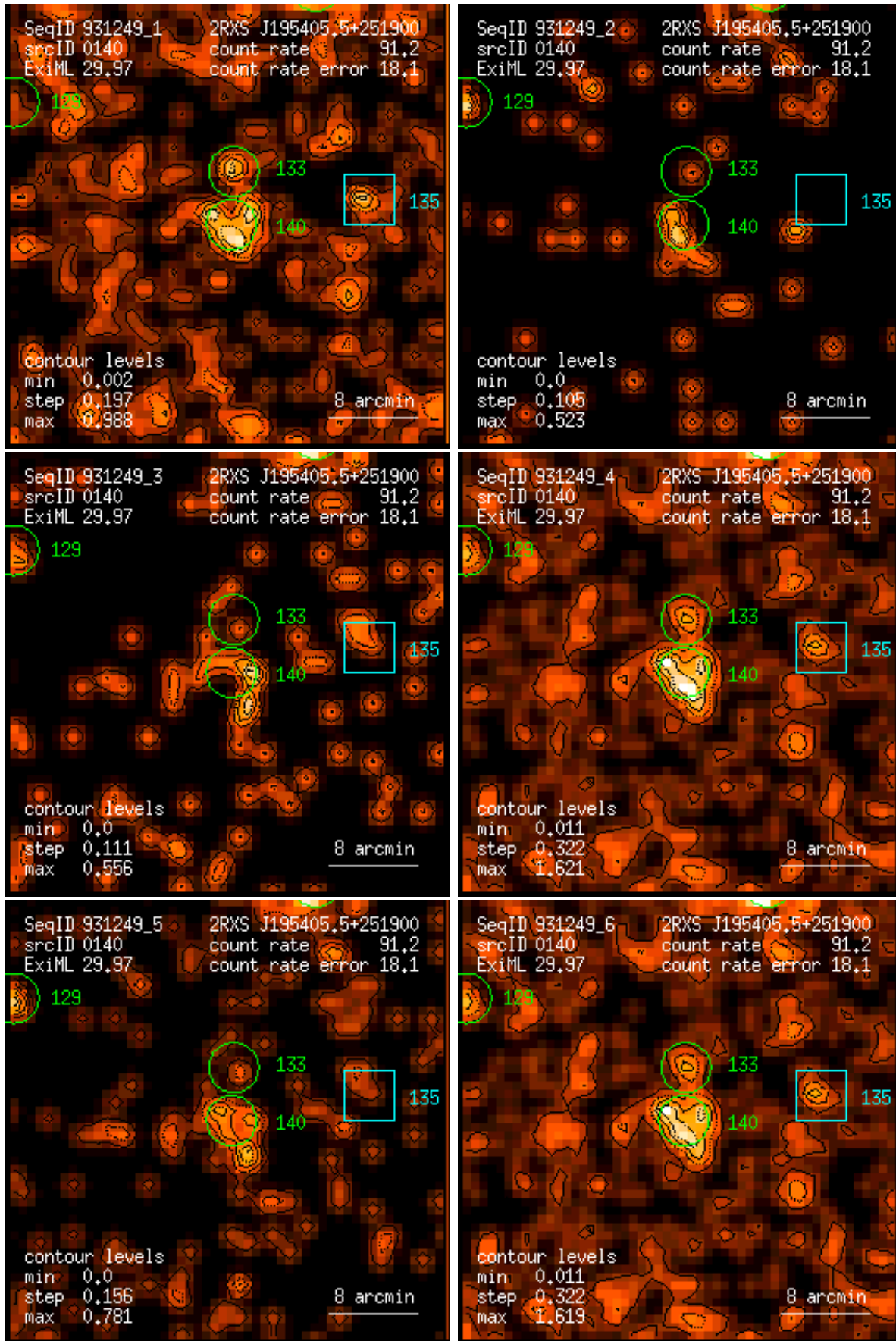
Figure 140: RASS 931249: detection 0140: band rate images, Gaussian filter: (1) PSPC channels 11 – 41, (2) 52 – 90, (3) 91 – 201, (4) 11 – 235, (5) 52 – 201, (6) 11 – 201. Broad band rates in counts/ks. Band rate contour levels in counts/ks/arcmin 2 .
