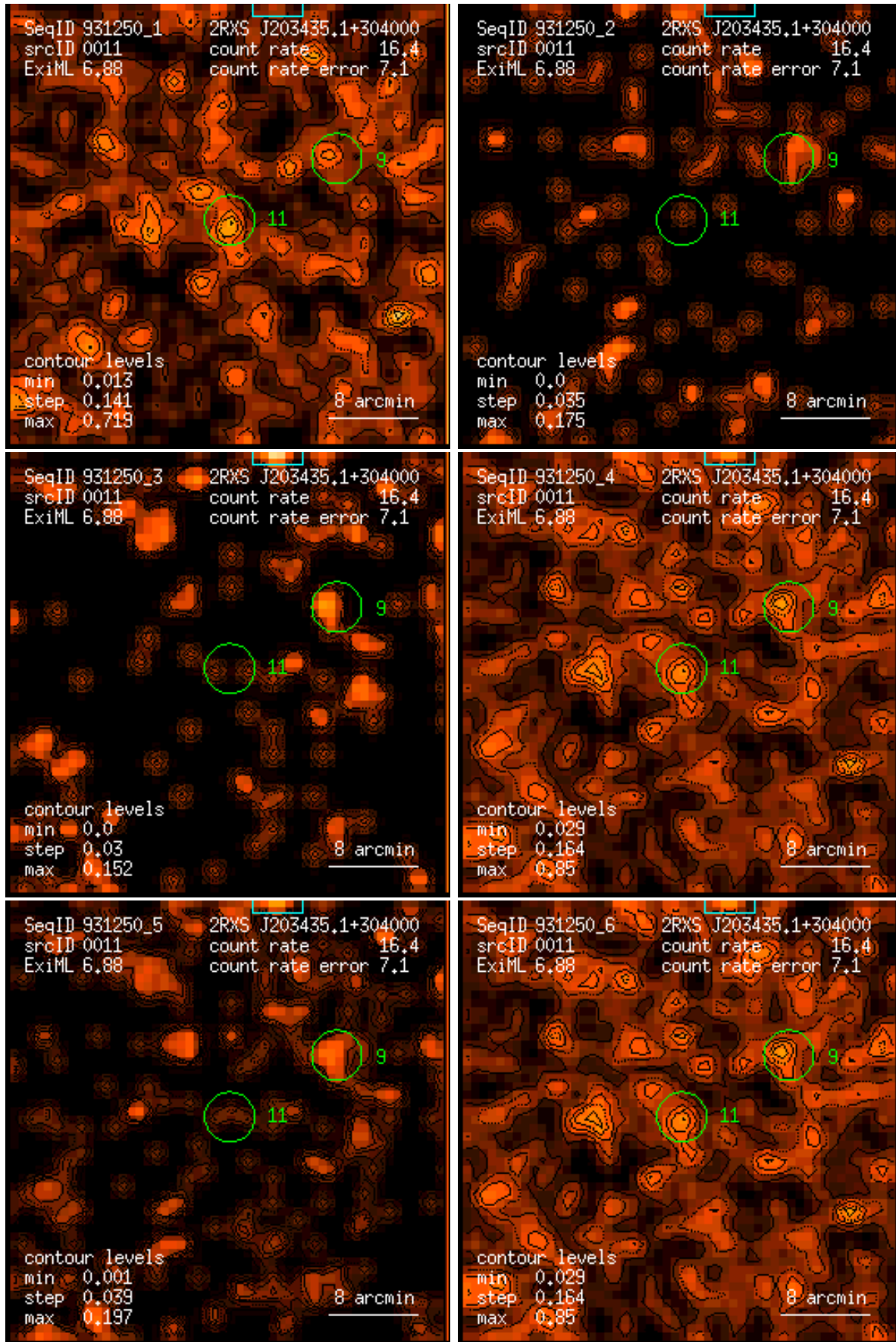
Figure 11: RASS 931250: detection 0011: band rate images, Gaussian filter: (1) PSPC channels 11 – 41, (2) 52 – 90, (3) 91 – 201, (4) 11 – 235, (5) 52 – 201, (6) 11 – 201. Broad band rates in counts/ks. Band rate contour levels in counts/ks/arcmin 2 .
