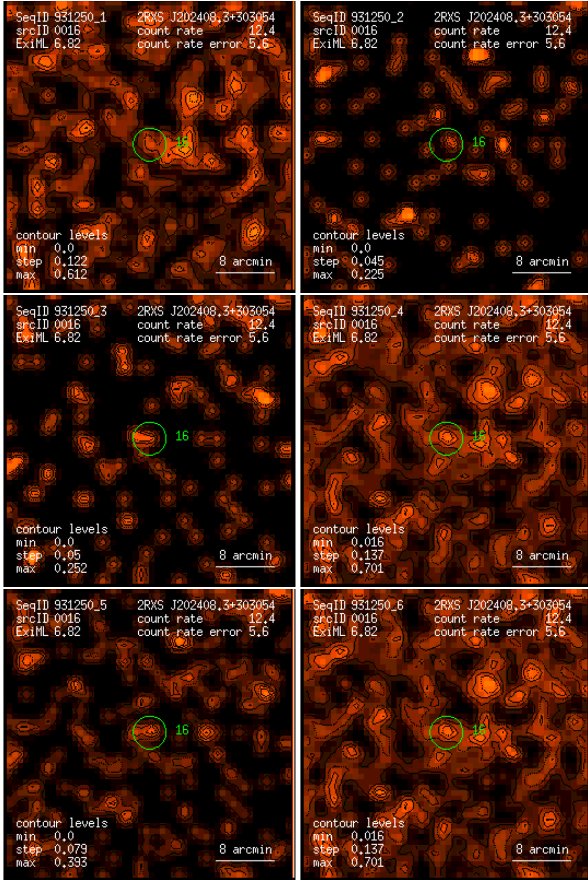
Figure 16: RASS 931250: detection 0016: band rate images, Gaussian filter: (1) PSPC channels 11 – 41, (2) 52 – 90, (3) 91 – 201, (4) 11 – 235, (5) 52 – 201, (6) 11 – 201. Broad band rates in counts/ks. Band rate contour levels in counts/ks/arcmin 2 .
