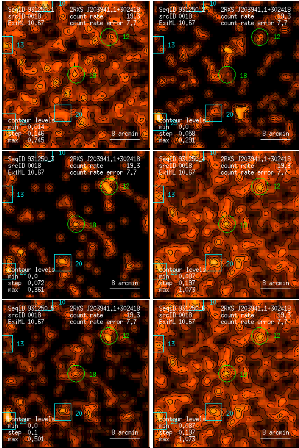
Figure 18: RASS 931250: detection 0018: band rate images, Gaussian filter: (1) PSPC channels 11 – 41, (2) 52 – 90, (3) 91 – 201, (4) 11 – 235, (5) 52 – 201, (6) 11 – 201. Broad band rates in counts/ks. Band rate contour levels in counts/ks/arcmin 2 .
