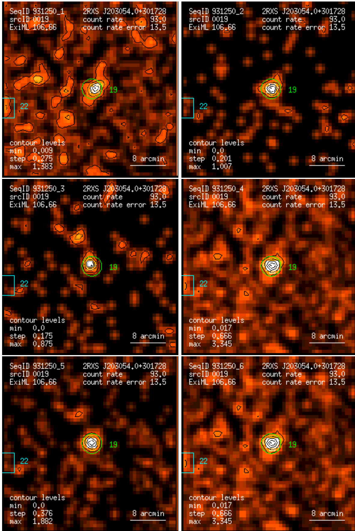
Figure 19: RASS 931250: detection 0019: band rate images, Gaussian filter: (1) PSPC channels 11 – 41, (2) 52 – 90, (3) 91 – 201, (4) 11 – 235, (5) 52 – 201, (6) 11 – 201. Broad band rates in counts/ks. Band rate contour levels in counts/ks/arcmin 2 .
