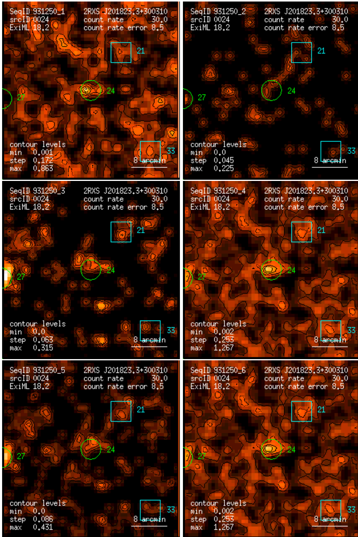
Figure 24: RASS 931250: detection 0024: band rate images, Gaussian filter: (1) PSPC channels 11 – 41, (2) 52 – 90, (3) 91 – 201, (4) 11 – 235, (5) 52 – 201, (6) 11 – 201. Broad band rates in counts/ks. Band rate contour levels in counts/ks/arcmin 2 .
