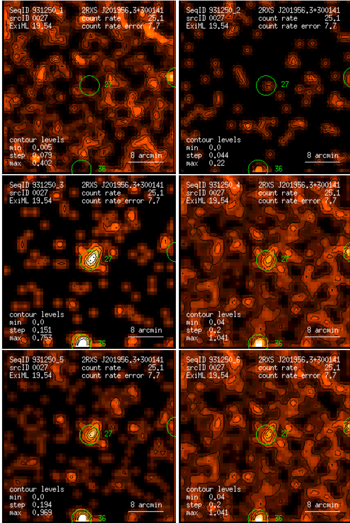
Figure 27: RASS 931250: detection 0027: band rate images, Gaussian filter: (1) PSPC channels 11 – 41, (2) 52 – 90, (3) 91 – 201, (4) 11 – 235, (5) 52 – 201, (6) 11 – 201. Broad band rates in counts/ks. Band rate contour levels in counts/ks/arcmin 2 .
