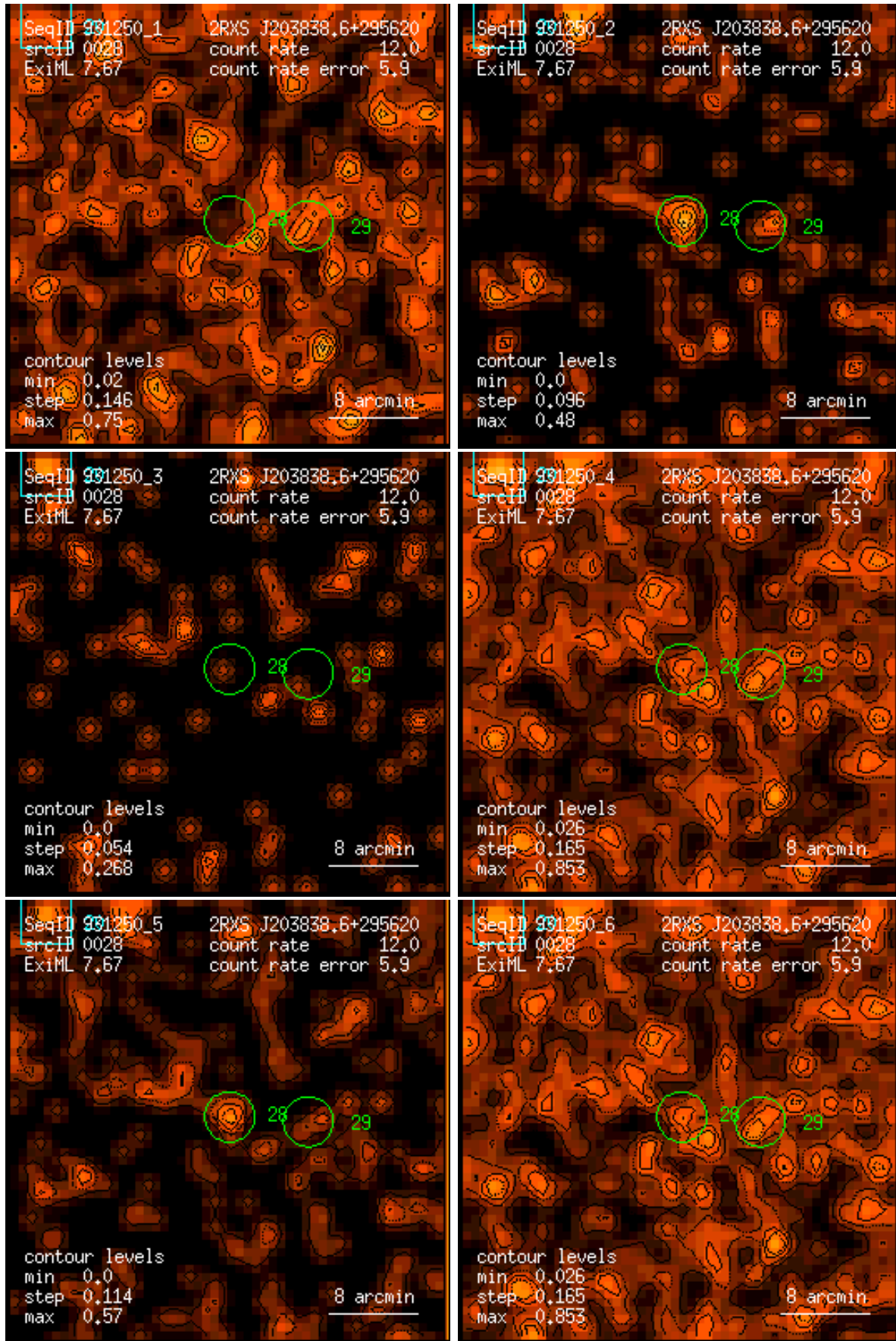
Figure 28: RASS 931250: detection 0028: band rate images, Gaussian filter: (1) PSPC channels 11 – 41, (2) 52 – 90, (3) 91 – 201, (4) 11 – 235, (5) 52 – 201, (6) 11 – 201. Broad band rates in counts/ks. Band rate contour levels in counts/ks/arcmin 2 .
