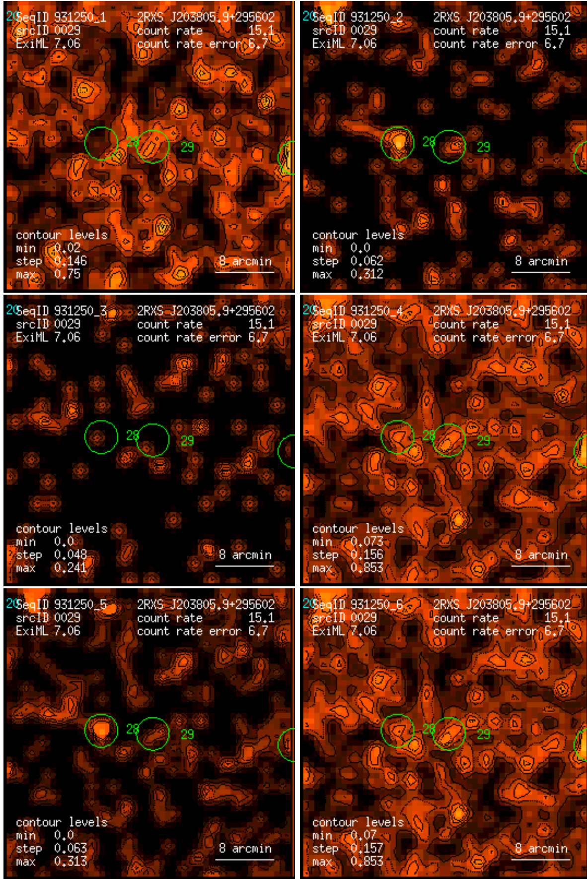
Figure 29: RASS 931250: detection 0029: band rate images, Gaussian filter: (1) PSPC channels 11 – 41, (2) 52 – 90, (3) 91 – 201, (4) 11 – 235, (5) 52 – 201, (6) 11 – 201. Broad band rates in counts/ks. Band rate contour levels in counts/ks/arcmin 2 .
