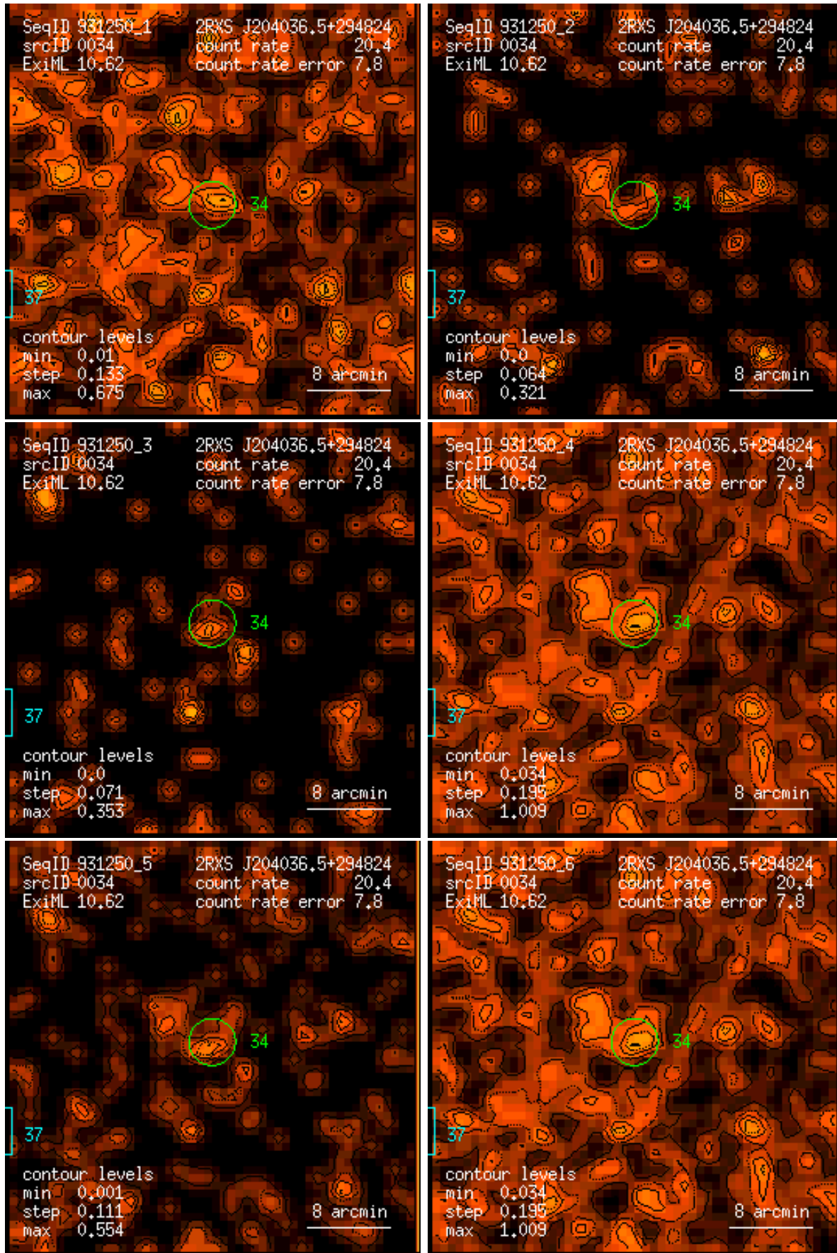
Figure 34: RASS 931250: detection 0034: band rate images, Gaussian filter: (1) PSPC channels 11 – 41, (2) 52 – 90, (3) 91 – 201, (4) 11 – 235, (5) 52 – 201, (6) 11 – 201. Broad band rates in counts/ks. Band rate contour levels in counts/ks/arcmin 2 .
