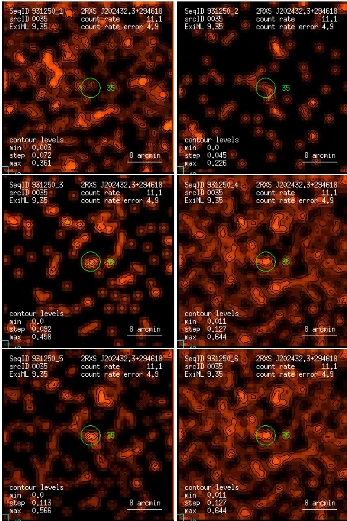
Figure 35: RASS 931250: detection 0035: band rate images, Gaussian filter: (1) PSPC channels 11 – 41, (2) 52 – 90, (3) 91 – 201, (4) 11 – 235, (5) 52 – 201, (6) 11 – 201. Broad band rates in counts/ks. Band rate contour levels in counts/ks/arcmin 2 .
