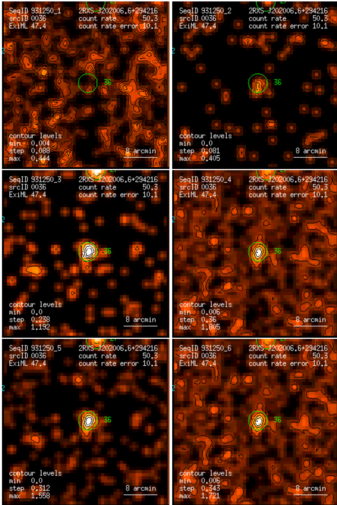
Figure 36: RASS 931250: detection 0036: band rate images, Gaussian filter: (1) PSPC channels 11 – 41, (2) 52 – 90, (3) 91 – 201, (4) 11 – 235, (5) 52 – 201, (6) 11 – 201. Broad band rates in counts/ks. Band rate contour levels in counts/ks/arcmin 2 .
