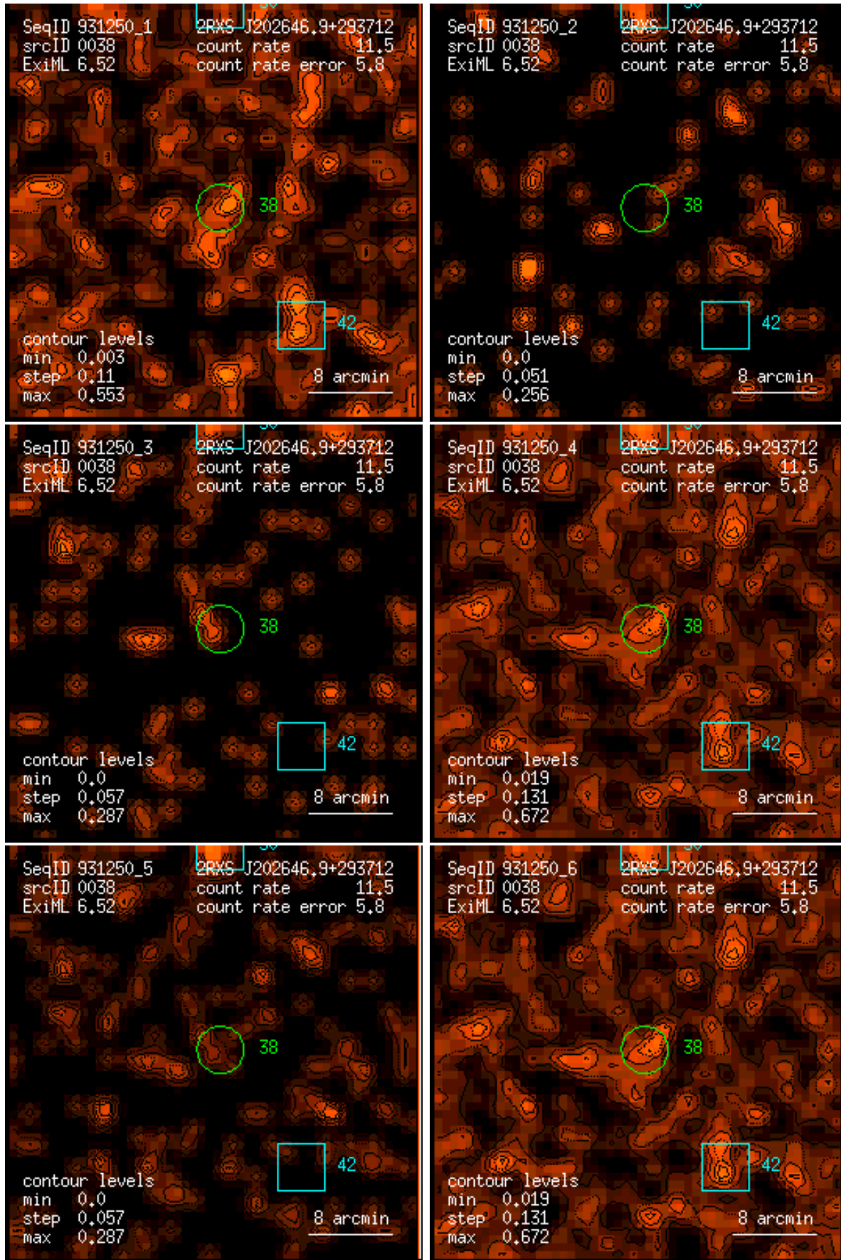
Figure 38: RASS 931250: detection 0038: band rate images, Gaussian filter: (1) PSPC channels 11 – 41, (2) 52 – 90, (3) 91 – 201, (4) 11 – 235, (5) 52 – 201, (6) 11 – 201. Broad band rates in counts/ks. Band rate contour levels in counts/ks/arcmin 2 .
