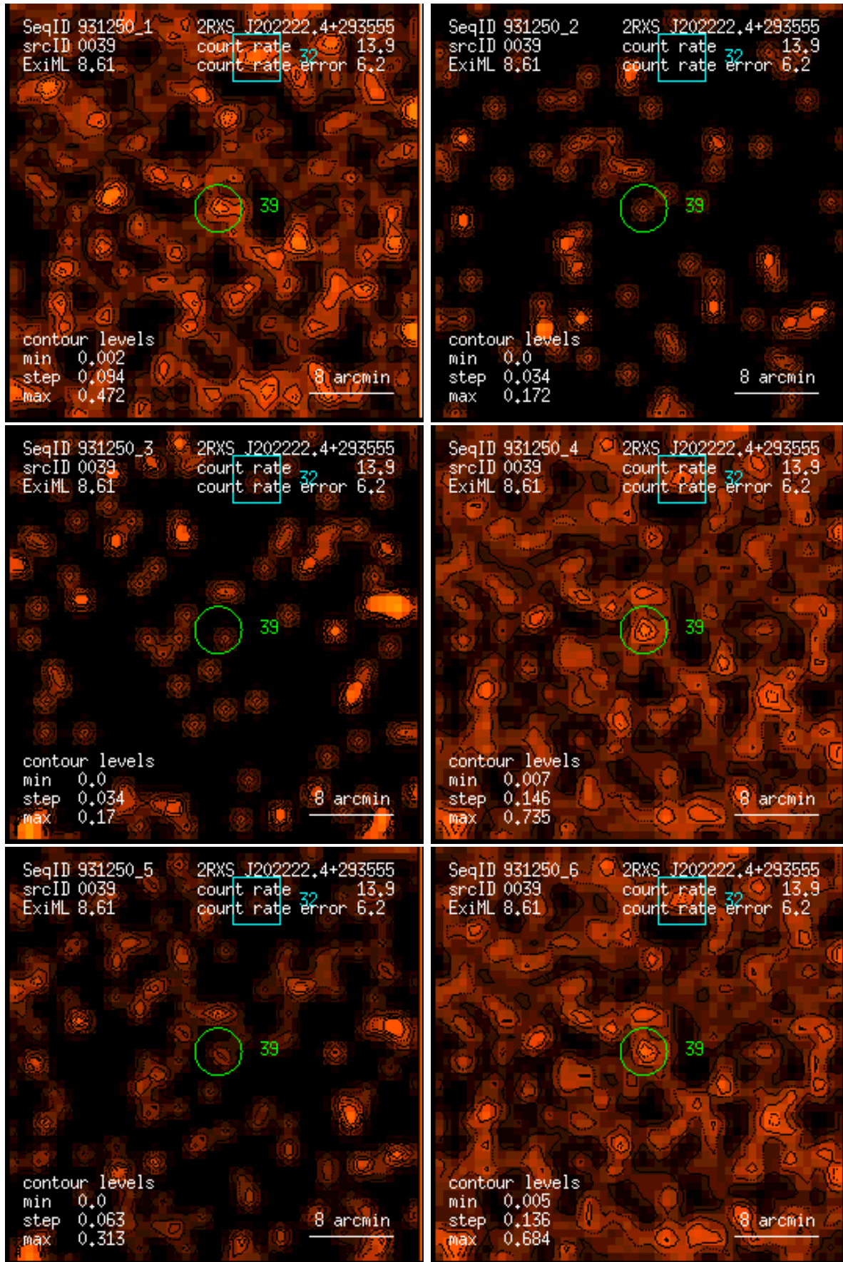
Figure 39: RASS 931250: detection 0039: band rate images, Gaussian filter: (1) PSPC channels 11 – 41, (2) 52 – 90, (3) 91 – 201, (4) 11 – 235, (5) 52 – 201, (6) 11 – 201. Broad band rates in counts/ks. Band rate contour levels in counts/ks/arcmin 2 .
