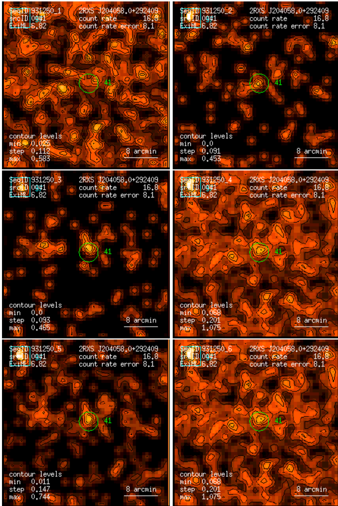
Figure 41: RASS 931250: detection 0041: band rate images, Gaussian filter: (1) PSPC channels 11 – 41, (2) 52 – 90, (3) 91 – 201, (4) 11 – 235, (5) 52 – 201, (6) 11 – 201. Broad band rates in counts/ks. Band rate contour levels in counts/ks/arcmin 2 .
