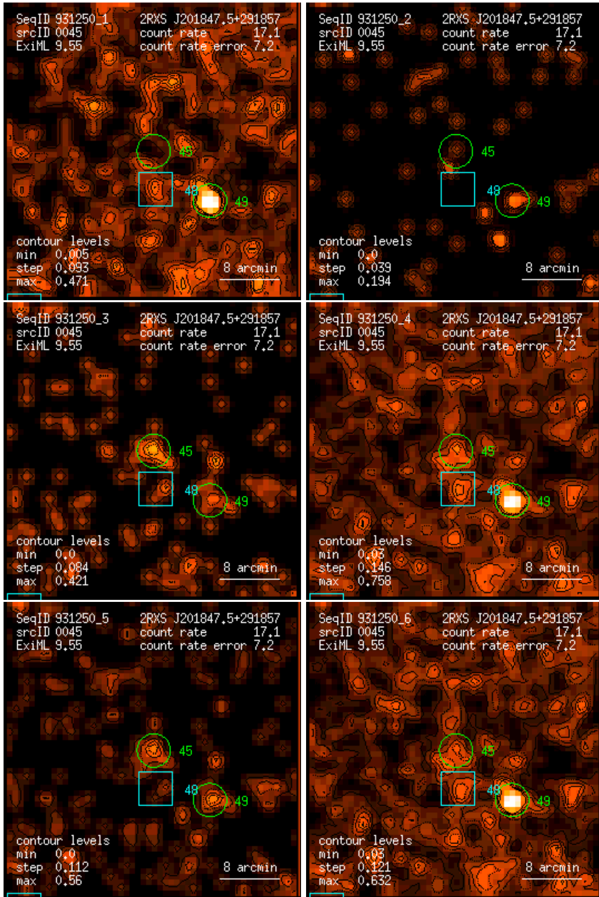
Figure 45: RASS 931250: detection 0045: band rate images, Gaussian filter: (1) PSPC channels 11 – 41, (2) 52 – 90, (3) 91 – 201, (4) 11 – 235, (5) 52 – 201, (6) 11 – 201. Broad band rates in counts/ks. Band rate contour levels in counts/ks/arcmin 2 .
