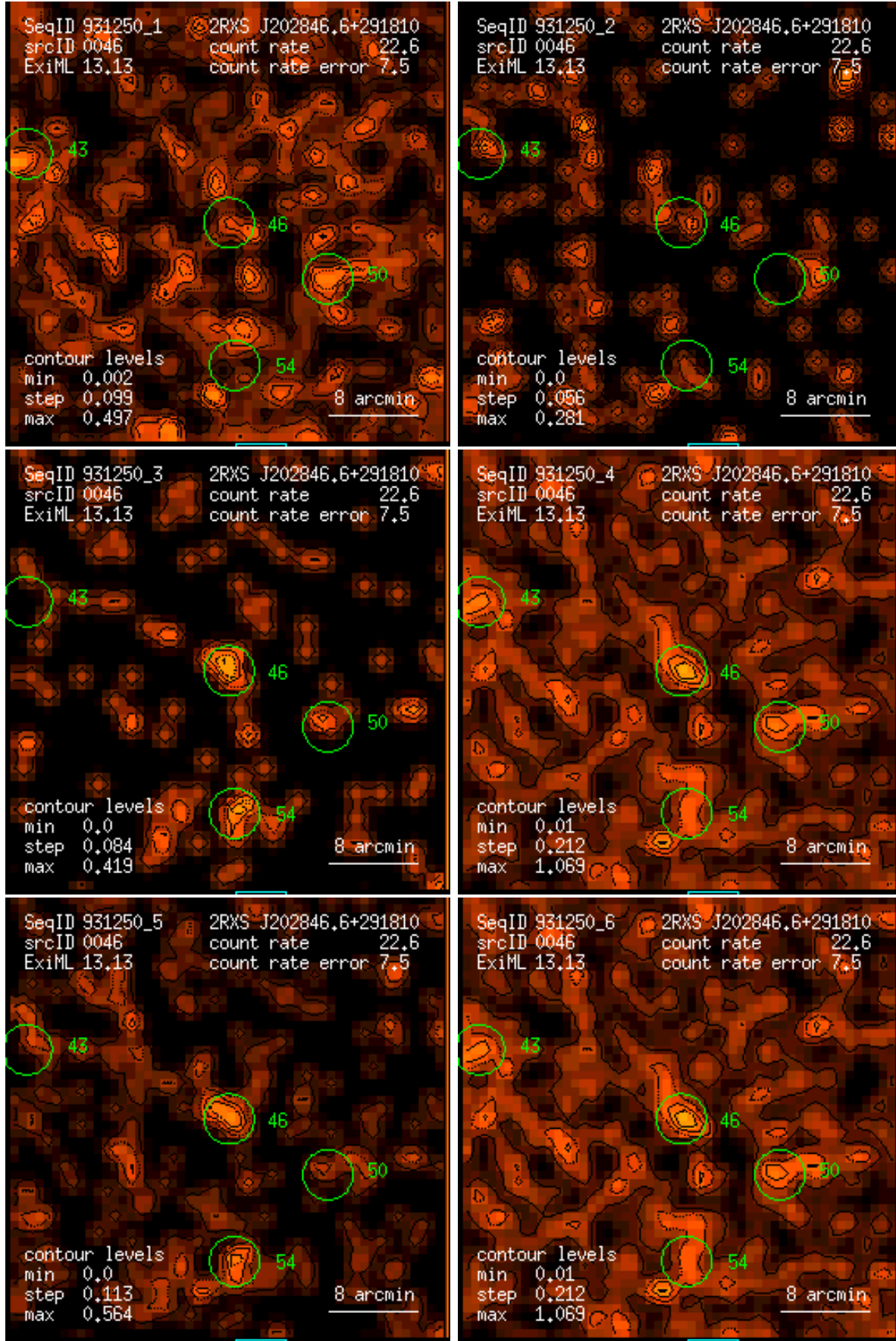
Figure 46: RASS 931250: detection 0046: band rate images, Gaussian filter: (1) PSPC channels 11 – 41, (2) 52 – 90, (3) 91 – 201, (4) 11 – 235, (5) 52 – 201, (6) 11 – 201. Broad band rates in counts/ks. Band rate contour levels in counts/ks/arcmin 2 .
