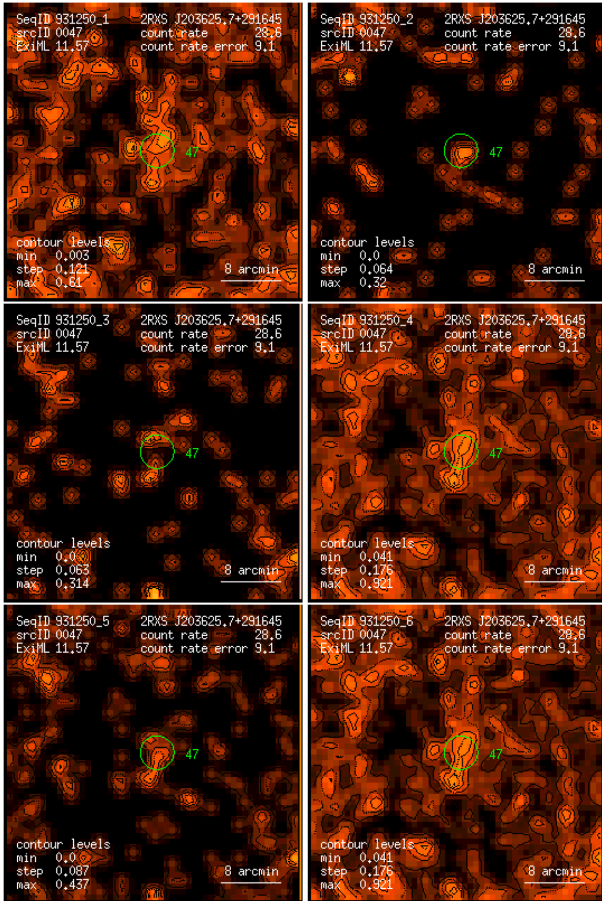
Figure 47: RASS 931250: detection 0047: band rate images, Gaussian filter: (1) PSPC channels 11 – 41, (2) 52 – 90, (3) 91 – 201, (4) 11 – 235, (5) 52 – 201, (6) 11 – 201. Broad band rates in counts/ks. Band rate contour levels in counts/ks/arcmin 2 .
