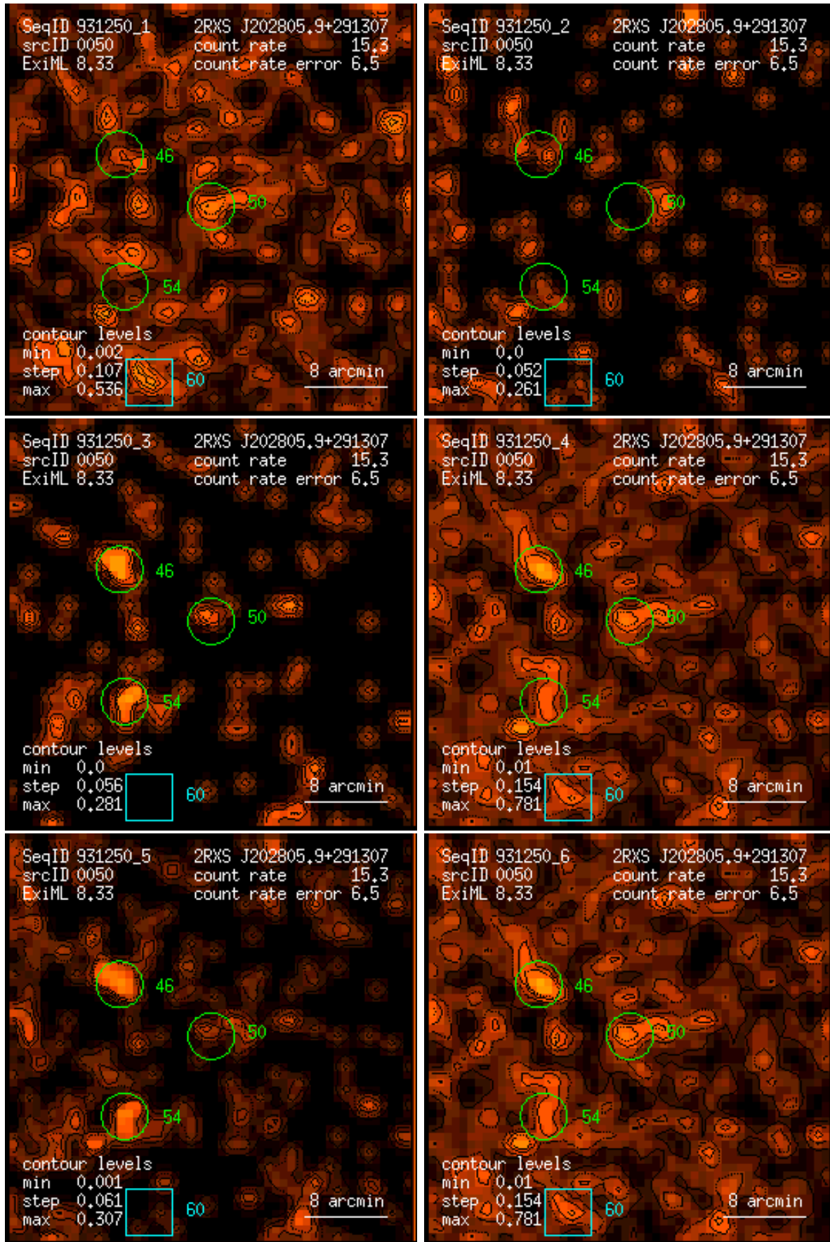
Figure 50: RASS 931250: detection 0050: band rate images, Gaussian filter: (1) PSPC channels 11 – 41, (2) 52 – 90, (3) 91 – 201, (4) 11 – 235, (5) 52 – 201, (6) 11 – 201. Broad band rates in counts/ks. Band rate contour levels in counts/ks/arcmin 2 .
