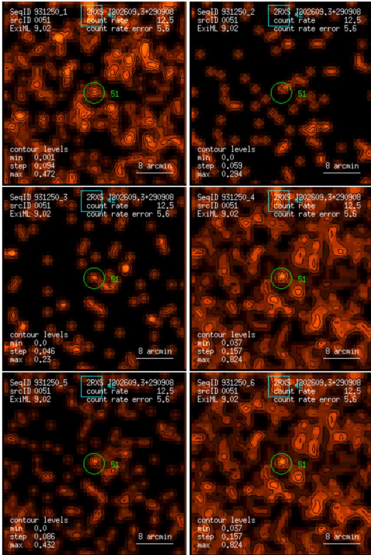
Figure 51: RASS 931250: detection 0051: band rate images, Gaussian filter: (1) PSPC channels 11 – 41, (2) 52 – 90, (3) 91 – 201, (4) 11 – 235, (5) 52 – 201, (6) 11 – 201. Broad band rates in counts/ks. Band rate contour levels in counts/ks/arcmin 2 .
