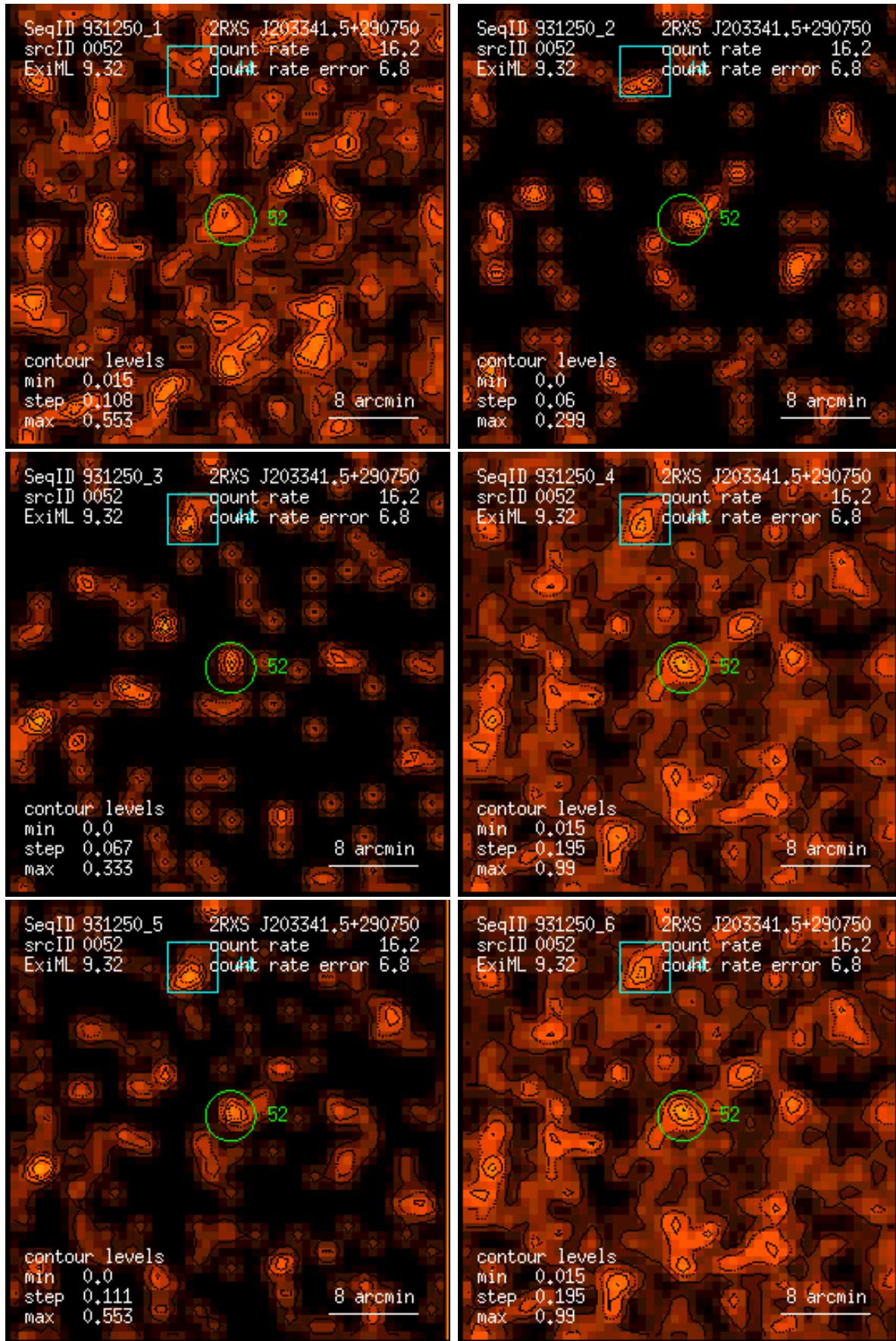
Figure 52: RASS 931250: detection 0052: band rate images, Gaussian filter: (1) PSPC channels 11 – 41, (2) 52 – 90, (3) 91 – 201, (4) 11 – 235, (5) 52 – 201, (6) 11 – 201. Broad band rates in counts/ks. Band rate contour levels in counts/ks/arcmin 2 .
