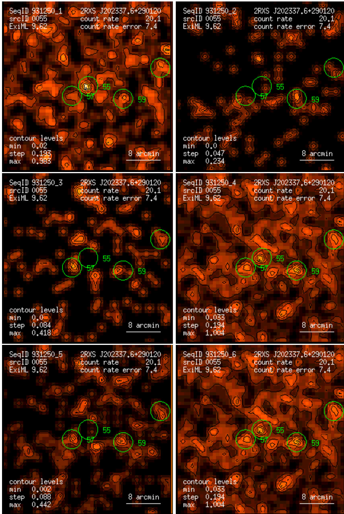
Figure 55: RASS 931250: detection 0055: band rate images, Gaussian filter: (1) PSPC channels 11 – 41, (2) 52 – 90, (3) 91 – 201, (4) 11 – 235, (5) 52 – 201, (6) 11 – 201. Broad band rates in counts/ks. Band rate contour levels in counts/ks/arcmin 2 .
