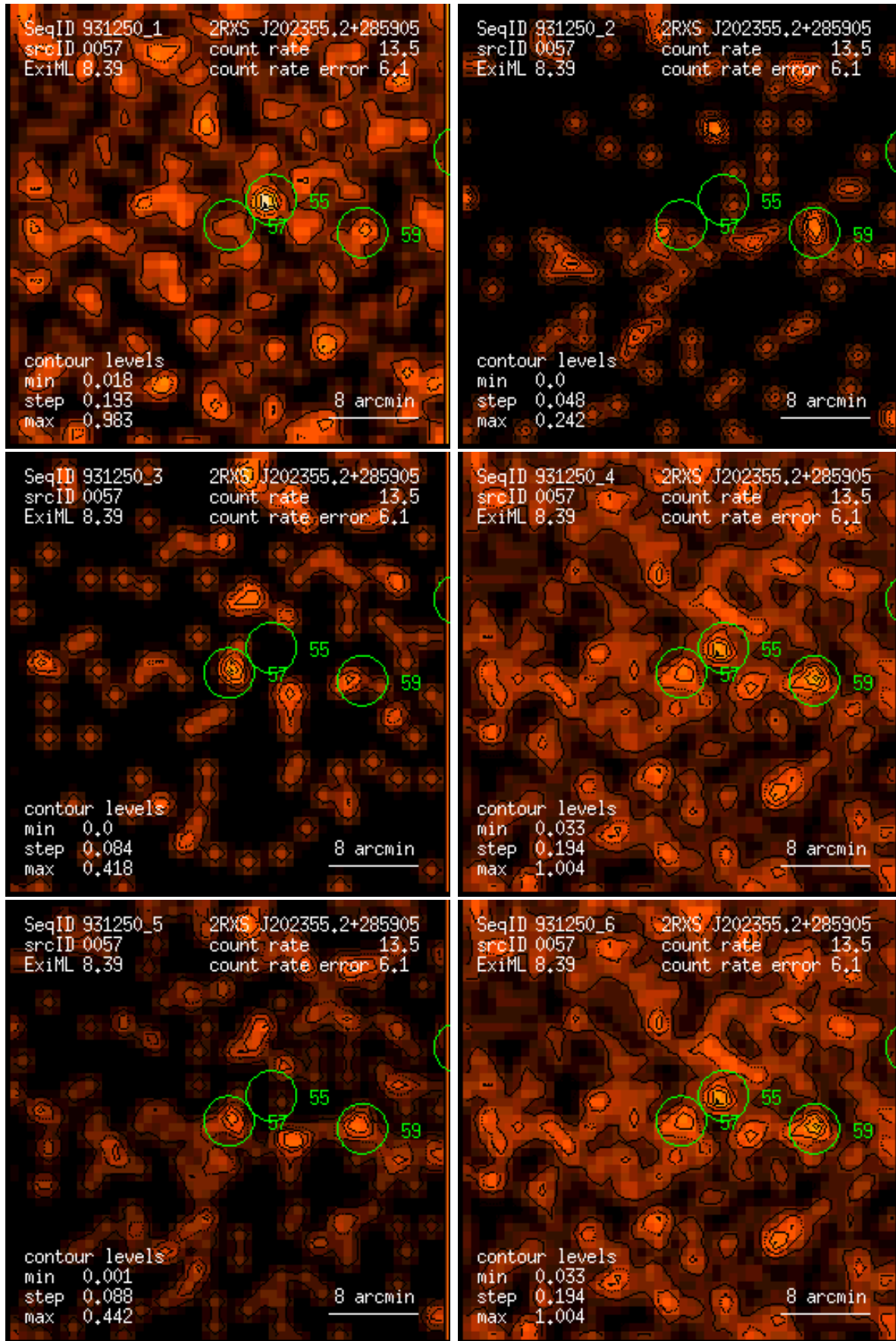
Figure 57: RASS 931250: detection 0057: band rate images, Gaussian filter: (1) PSPC channels 11 – 41, (2) 52 – 90, (3) 91 – 201, (4) 11 – 235, (5) 52 – 201, (6) 11 – 201. Broad band rates in counts/ks. Band rate contour levels in counts/ks/arcmin 2 .
