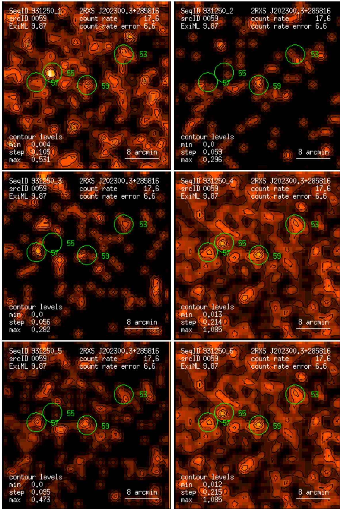
Figure 59: RASS 931250: detection 0059: band rate images, Gaussian filter: (1) PSPC channels 11 – 41, (2) 52 – 90, (3) 91 – 201, (4) 11 – 235, (5) 52 – 201, (6) 11 – 201. Broad band rates in counts/ks. Band rate contour levels in counts/ks/arcmin 2 .
