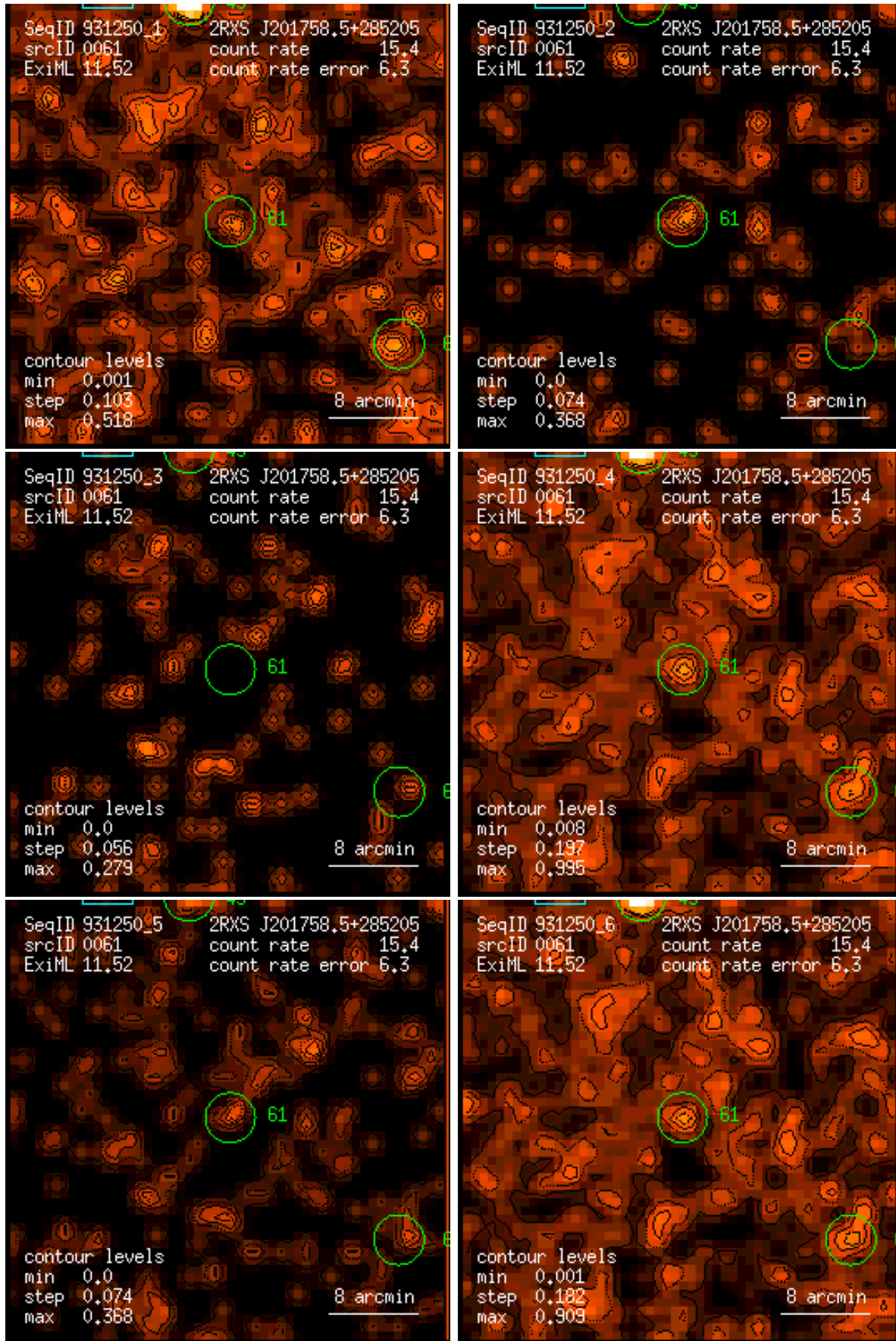
Figure 61: RASS 931250: detection 0061: band rate images, Gaussian filter: (1) PSPC channels 11 – 41, (2) 52 – 90, (3) 91 – 201, (4) 11 – 235, (5) 52 – 201, (6) 11 – 201. Broad band rates in counts/ks. Band rate contour levels in counts/ks/arcmin 2 .
